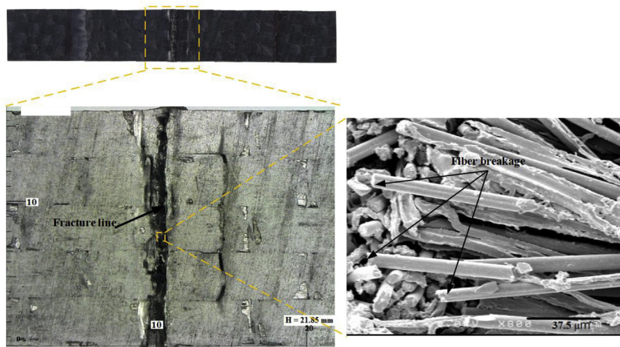
Fig. 14. Typical optical and SEM photographs for the fracture of MCLJ with 6 layers.
