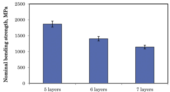
Fig. 11. Nominal bending strengths for SLJ with various layup numbers in the joint.
