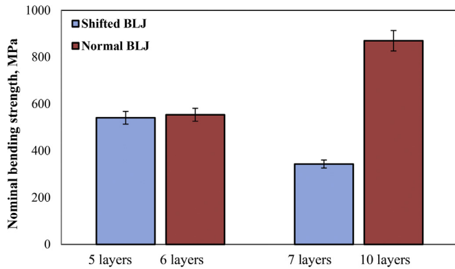
Fig. 6. Bending strength results for normal and shifted BLJ specimens.
