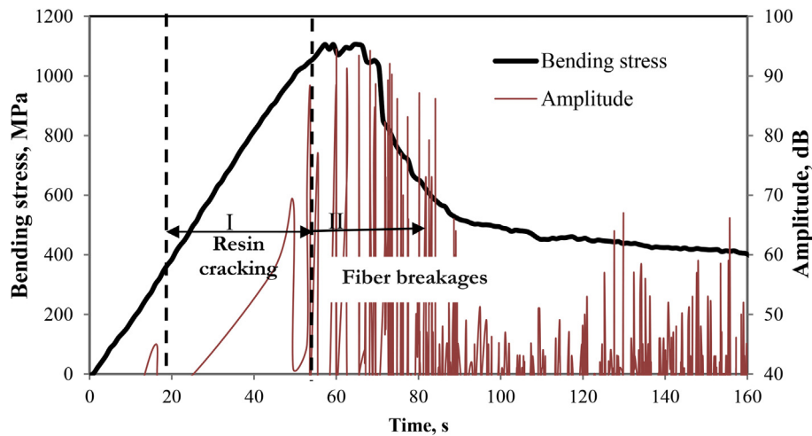
Fig. 8. Typical bending stress-time curve with accompanying AE amplitude for a shifted BLJ specimen of 5 fiber layers.
