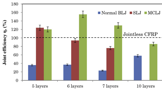
Fig. 16. Joint efficiencies for the various laminate joints as compared with jointless CFRP.
