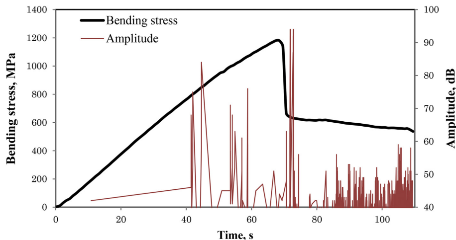
Fig. 7. Typical bending stress curve versus time with accompanying AE amplitudes for a normal BLJ specimen constructed of 6 fiber layers.
