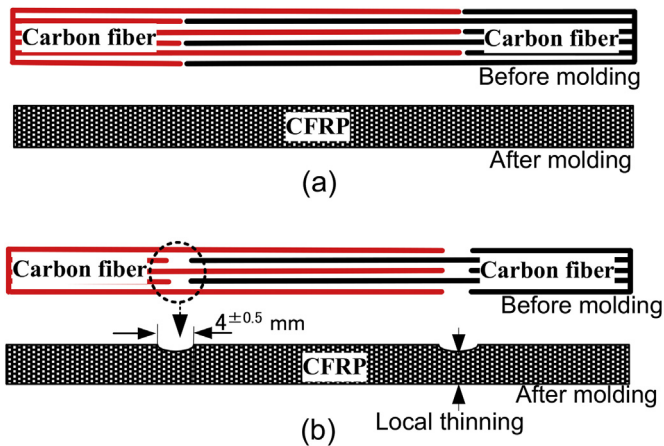
Fig. 3. Schematic drawing before and after molding for the (a) normal basic laminated joint (normal BLJ) and (b) shifted basic laminated joint (Shifted BLJ).
