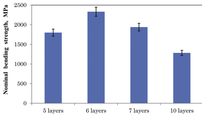
Fig. 13. Nominal bending strengths for MCLJ with various layers in the joint.
