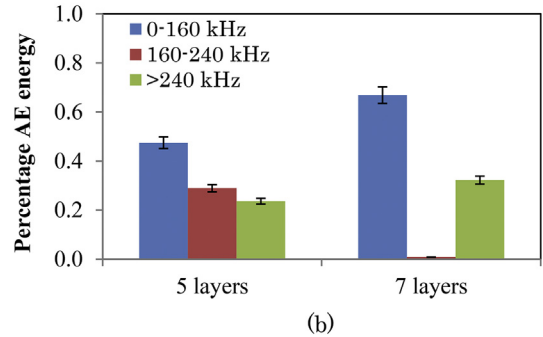
Fig. 10. Percentage data of AE energy for (a) normal BLJ and (b) shifted BLJ according to the three frequency bands.
