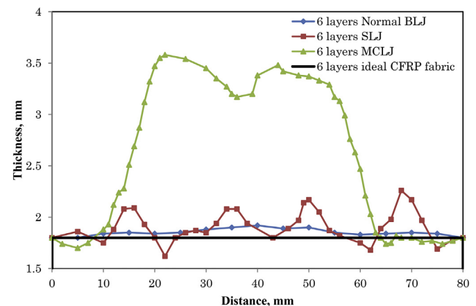
Fig. 5. Typical thickness profiles for the three types of joints and the jointless CFRP.
