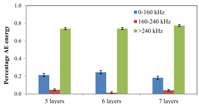
Fig. 12. Percentage data of AE energy for SLJ according to the three frequency bands.
