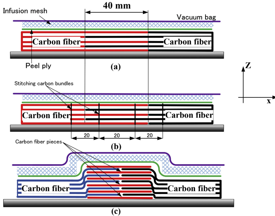
Fig. 2. (a) Basic laminated joint (BLJ). (b) Stitched laminated joint (SLJ). (c) Multiple-cover laminated joint (MCLJ).
