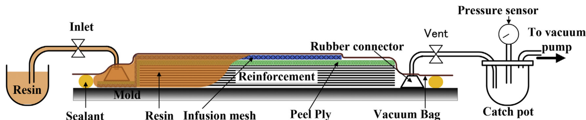
Fig. 1. Schematic diagram of the vacuum-assisted resin transfer molding (VARTM) process.
