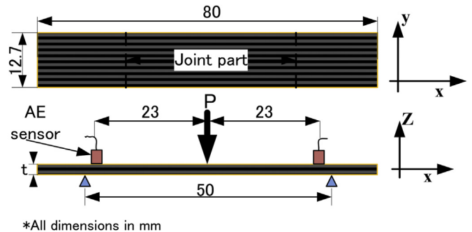
Fig. 4. Illustration of an adhesive joint specimen under the three-point bending test with acoustic emission (AE) monitoring.
