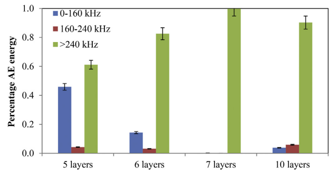
Fig. 15. Percentage data of AE energy for MCLJ according to the three frequency bands.
