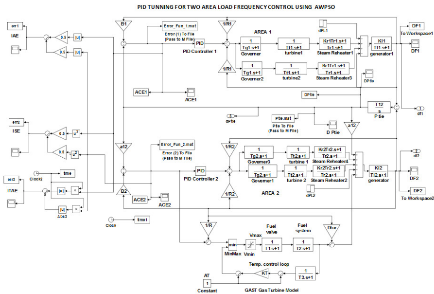
Figure 1: Model 1 Block Diagram
