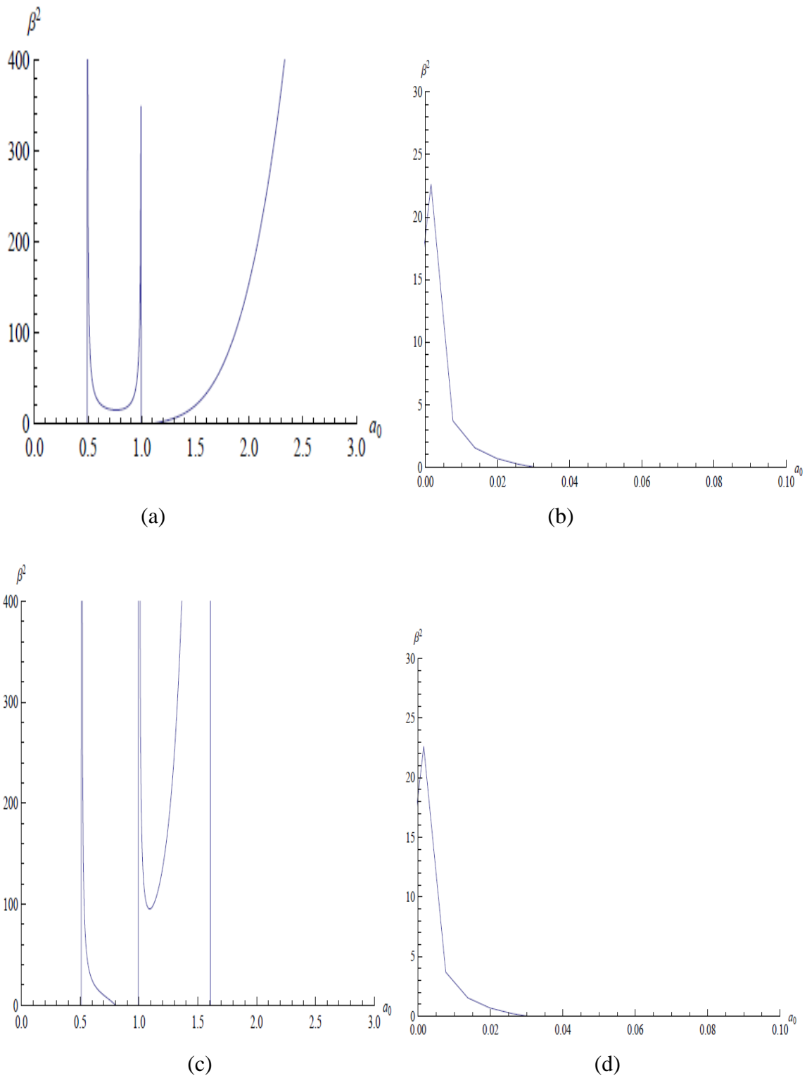
Figure 5. Stability regions TSW corresponding to \omega = 2 and the fixed value m = 1 : (a) \Lambda = -1, q = 1 , (b) \Lambda = -1, q = 0.5 , (c) \Lambda = 1, q = 1 , (d) \Lambda = 1, q = 0.5
