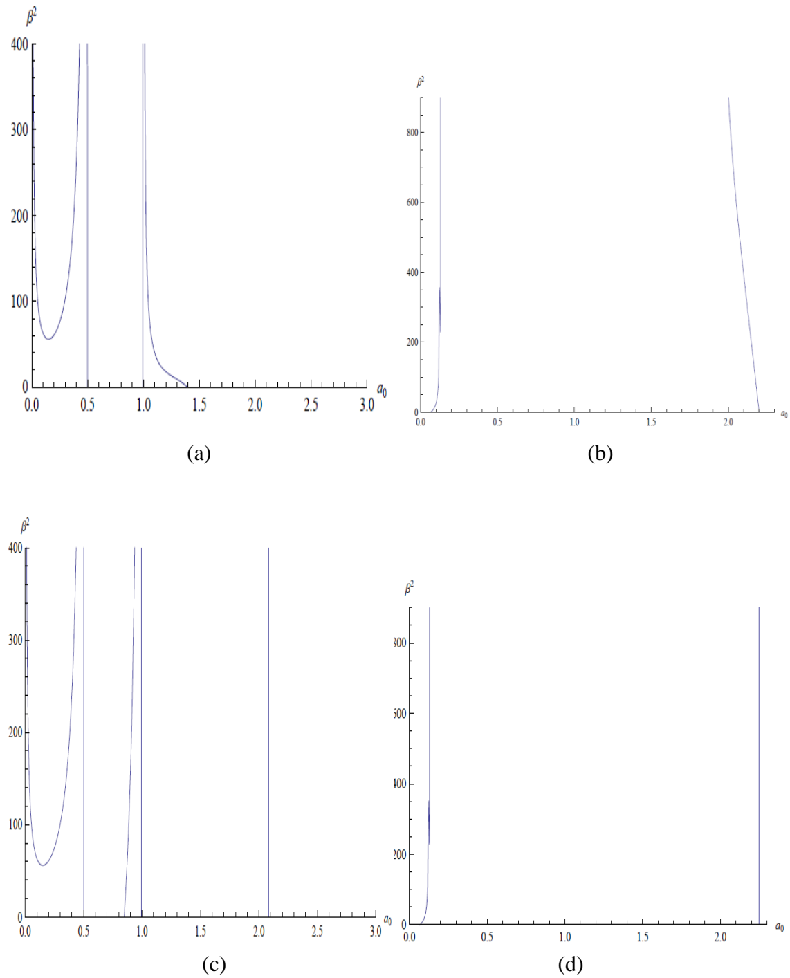
Figure 4. Stability regions TSW corresponding to \omega = 0.4 and the fixed value m = 1 : (a) \Lambda = -0.5 , q = 1 , (b) \Lambda = -0.5 , q = 0.5 , (c) \Lambda = 0.5 , q = 1 , (d) \Lambda = 0.5 , q = 0.5
