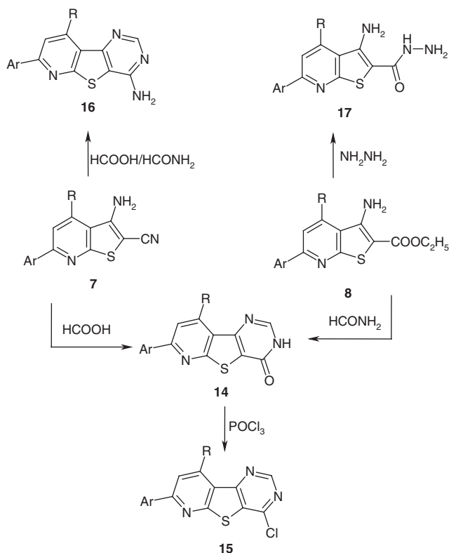
Scheme 3. Reactions of thienopyridines ( 7 , 8 ) with formic acid, formamide and hydrazine.
