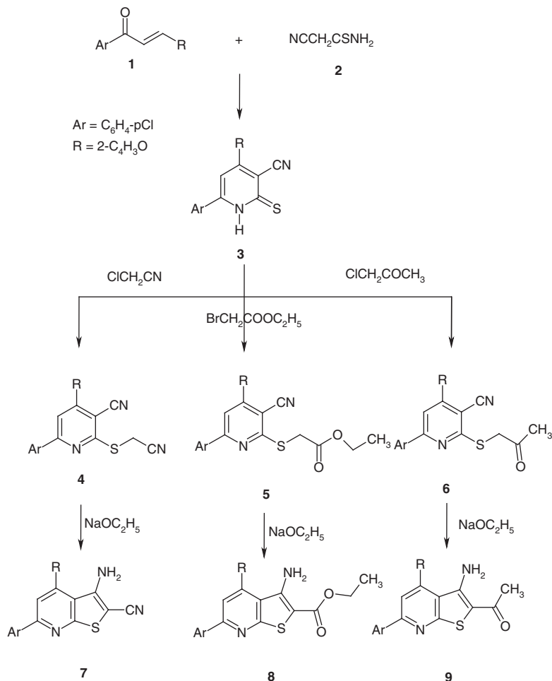
Scheme 1. Reactions of pyridinethione with chloroacetonitrile, ethyl bromoacetate and chloroacetone.
