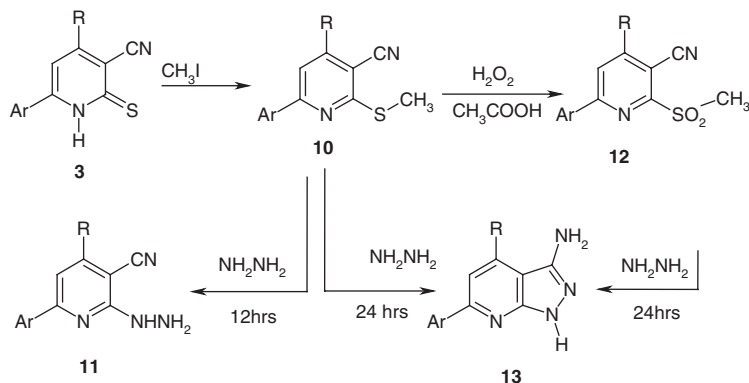
Scheme 2. Conversion of S-methyl derivative 10 to pyrazolopyridine derivative 13 .
