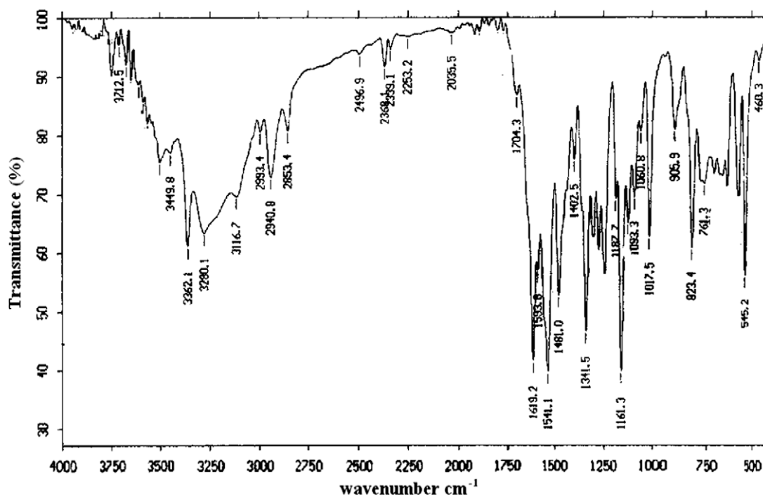
Figure 2 The FT-IR of Zn-glioclazide complex.
