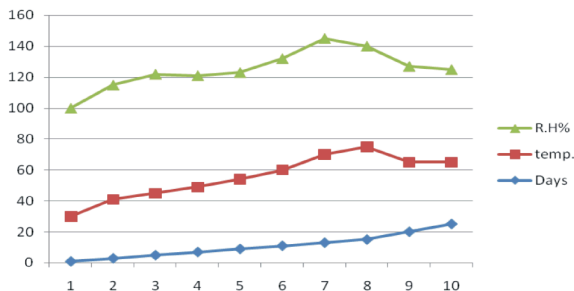
Fig. 1: Thermo-hygro profile of composting process. Days of sampling : 1, 3, 5, 7, 9, 11, 13, 15, 20 and 25 day
