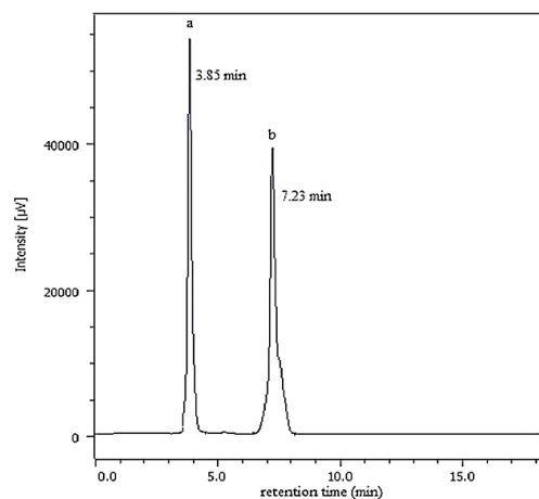
Figure 3. RP-HPLC chromatogram of 5 \mu\text{g/mL} (a) CDZ and 25 \mu\text{g/mL} (b) MVH using C18 (mobile phase consisted of 25 mM ammonium acetate buffer: acetonitrile in the ratio of 60:40 (v:v) (pH = 3)), flow rate of 1 mL/min at 260 nm.
