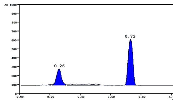
Figure 4. TLC-densitometric chromatogram of 2.5 \mu\text{g/band} MVH and 12 \mu\text{g/band} CDZ, respectively, using ethyl acetate: methanol (8:4, v:v) at 222 nm.
