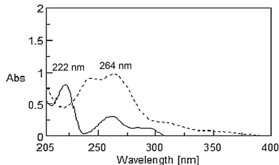
Figure 2. Zero-order spectra of 12 \mu\text{g/mL} of MVH (—) and 10 \mu\text{g/mL} of CDZ (...), separately in methanol
