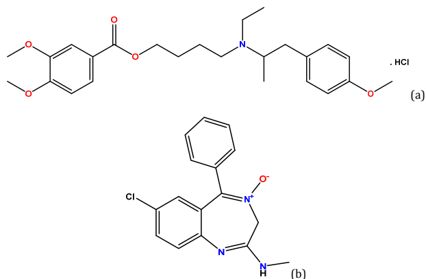
Figure 1. Chemical structure of mebeverine hydrochloride (a) and chlordiazepoxide (b).
