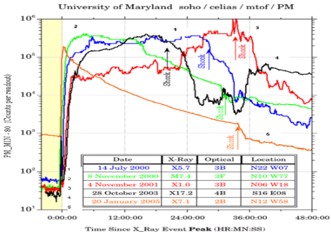
Fig. 3. Five distinguished X-ray flares chosen by SOHO team. X-ray and optical flare importance and locations on the sun are given. The number of event is given on diagram and on left of table.
