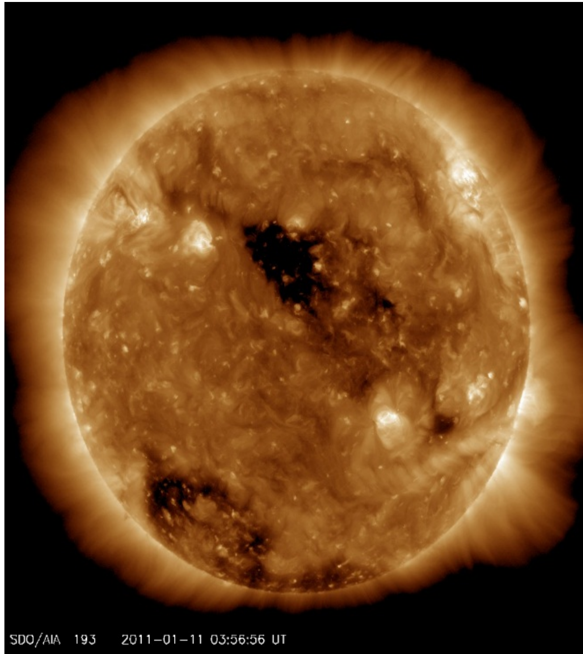
Fig. 5. Coronal Hole on 11 Jan 2011.
