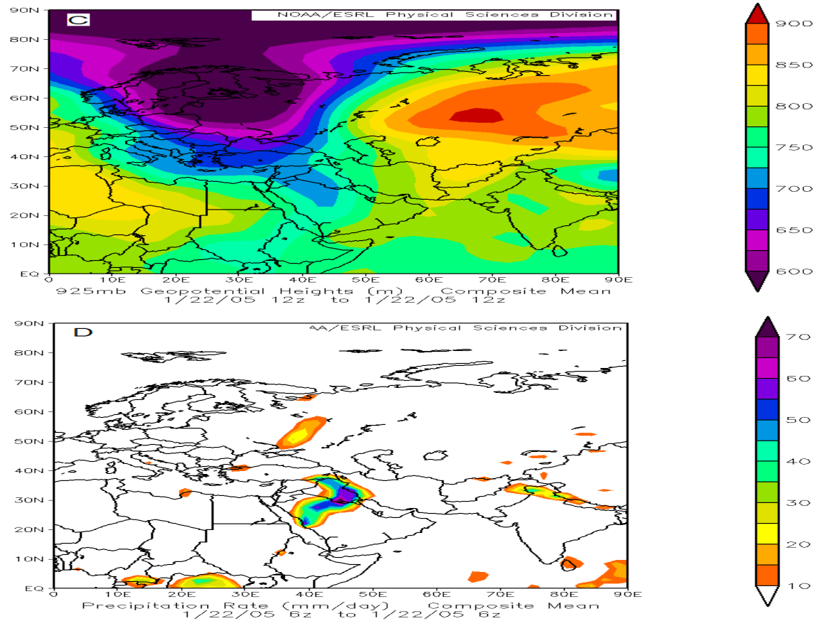
Fig. 4. 925 mb Geopotential height for the event of 22 January 2005 flash floods. A) 19 Jan 2005 map before CME hit the polar cap. B) 20 Jan map showing the position of CME hit of the polar atmosphere. C) 22 Jan at 12 UT map clearly indicates the extension of the low pressure region southward to Saudi Arabia passing by the Mediterranean Sea where the clouds were loaded with water. D) Precipitation rate map on 22 Jan 6h UT indicating excessive flash floods passing over Makkah Al-Mukaramah, Al-Madinah Al-Munawarah and Jeddah.
