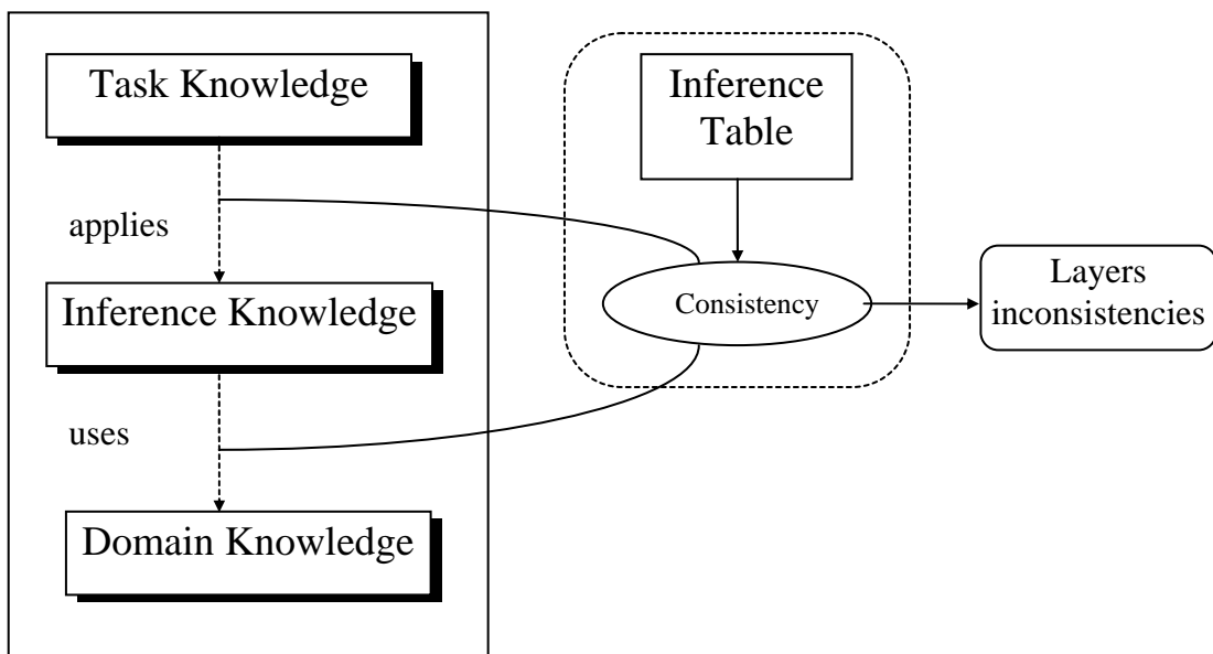
Figure 8: The structure of verification of the KADS Layers
