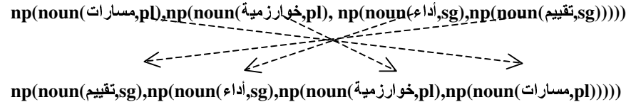
Figure 4. “of” transfer.
