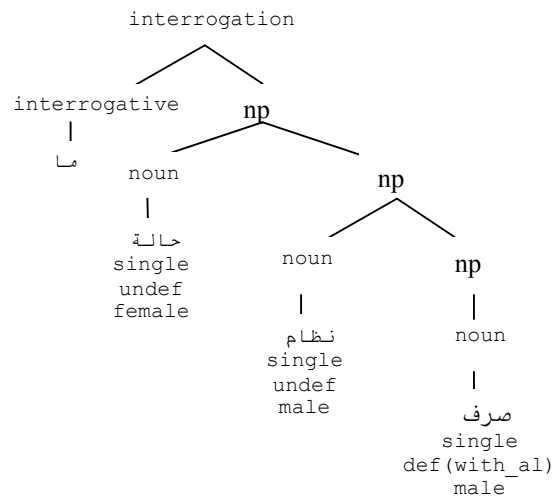
Fig 3. A parse tree for a simple sentence
