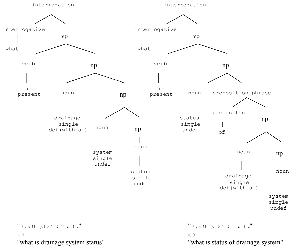
Fig. 5 A tree-to-tree transfer Example
