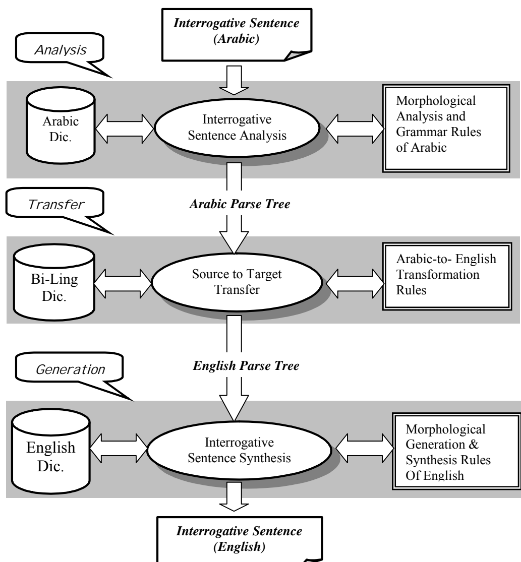
Fig 1. Overall Structure of Arabic-to- English Interrogative sentence Translator
