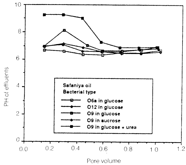
Fig. 8. Effect of bacterial types on pH of effluents.
