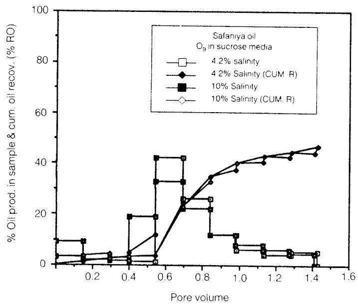
Fig. 14. Effect of salinity on production history for O_2 in sucrose solution.
