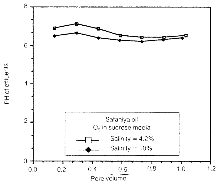
Fig. 15. PH of effluents as a function of pore volumes produced for O_2 in sucrose for different salinities.
