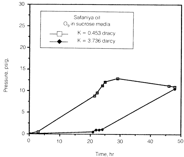
Fig. 13. Variation of model pressure with time after injecting O_9 in sucrose for different permeabilities.
