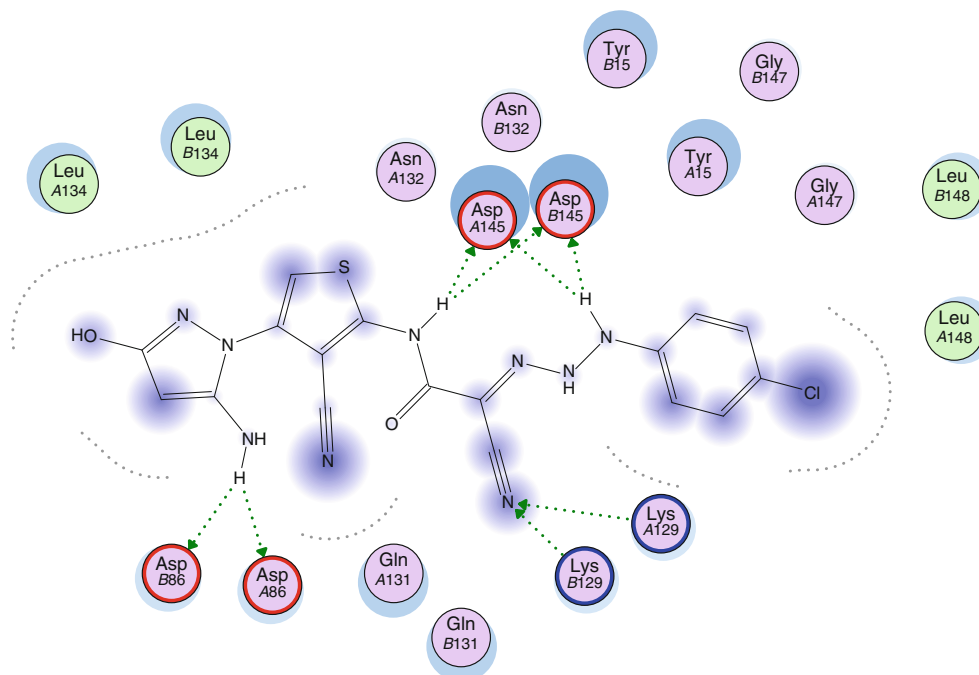
Fig. 5 Docking of compound 12c
