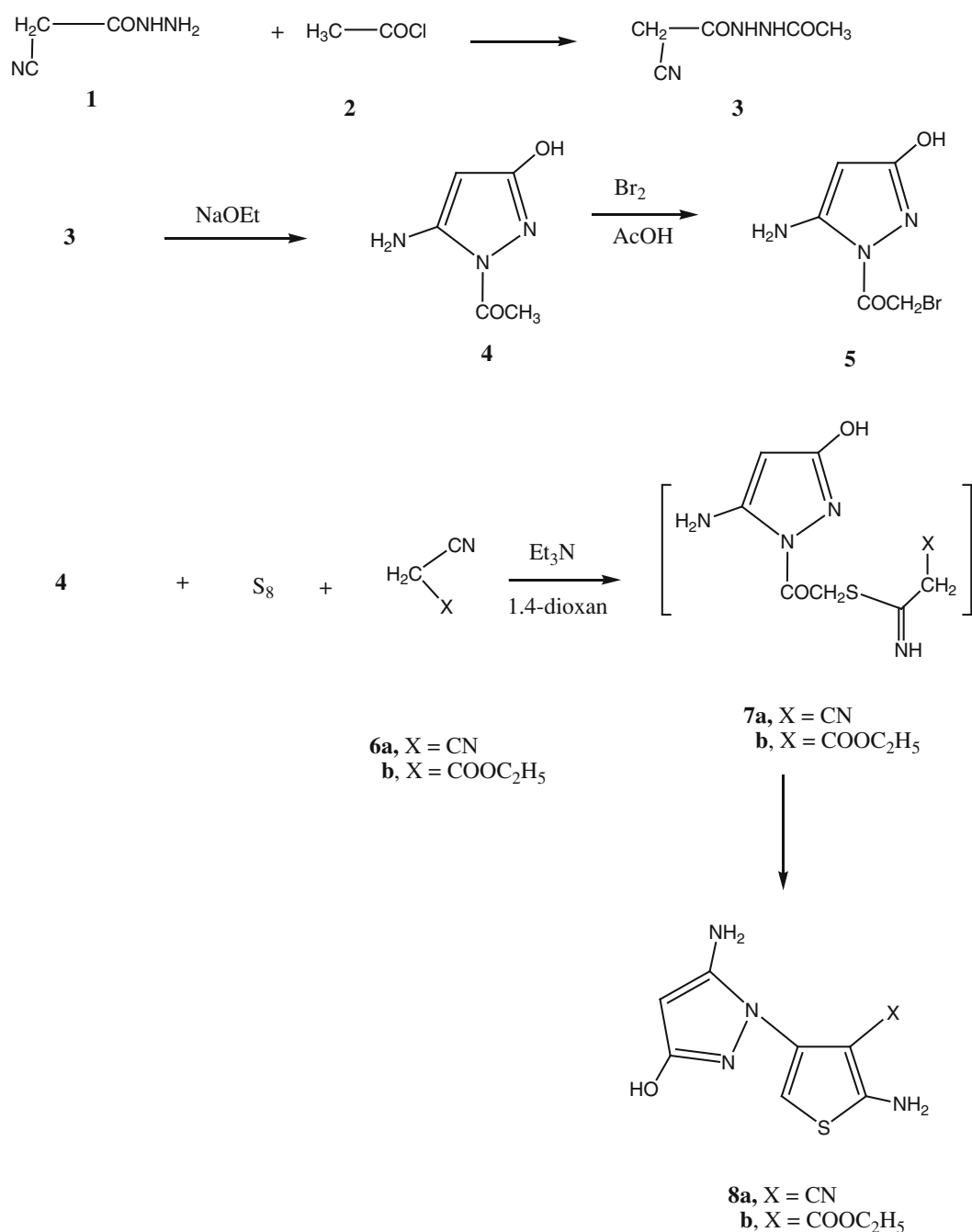
Scheme 1 Synthesis of compounds 3–8a,b
