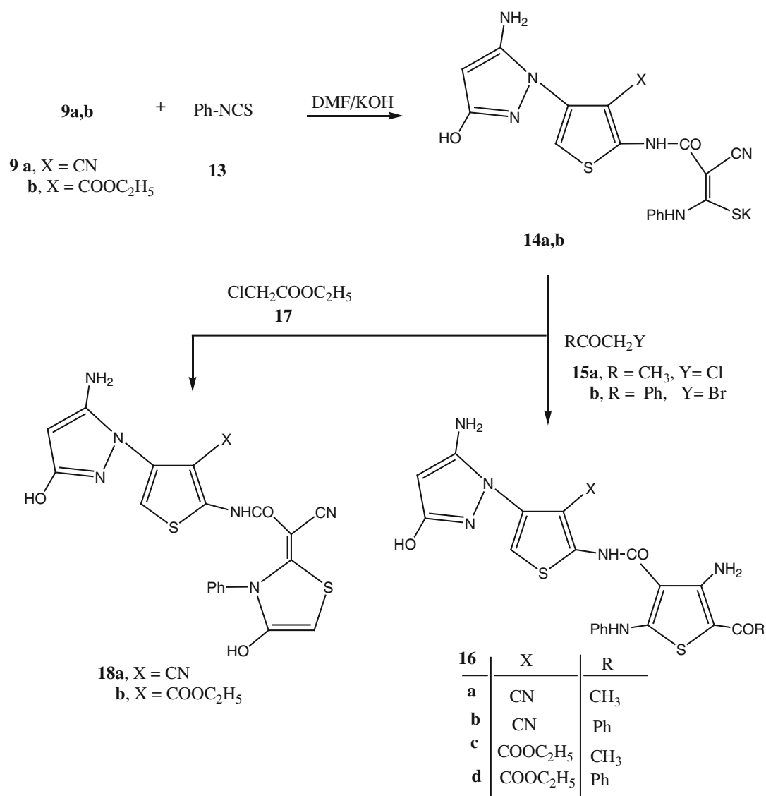
Scheme 3 Synthesis of compounds 14a,b–18a,b
