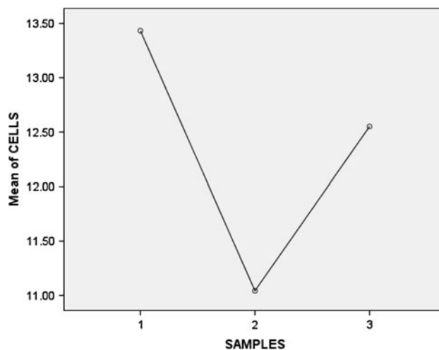
Fig. 4 Statistics ANOVA diagram
