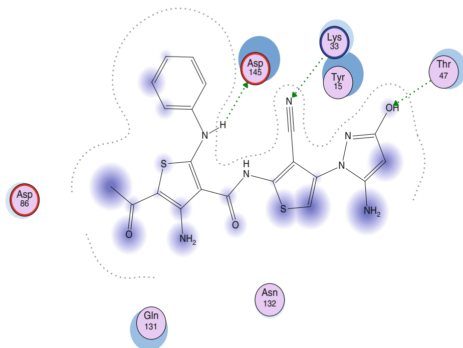
Fig. 7 Docking of compound 16a
