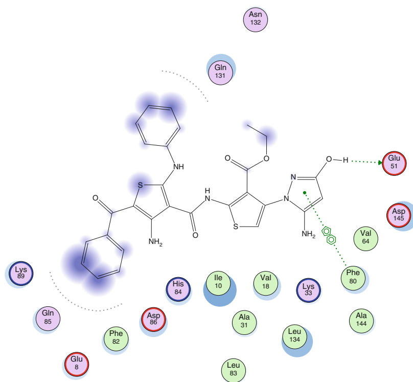
Fig. 8 Docking of compound 16d
