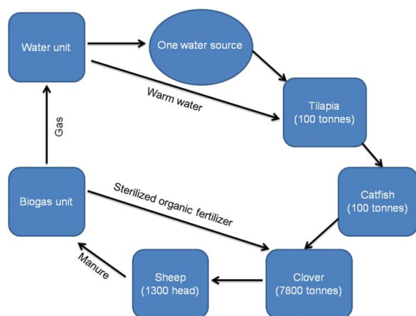
Figure 4. A diagram showing the sequential steps of integrated aquaculture in El-Keram farm using only one source of water, re-designed from the original source (El-Guindy, 2006).
