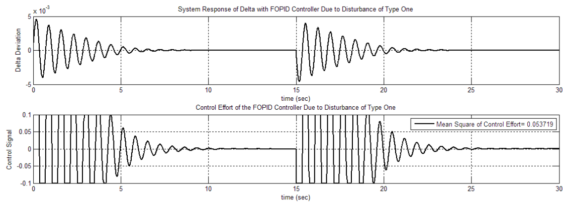
Figure 3. System response to 0.2 pu torque disturbance at ( P = 0.8 , Q = 0.3 )
