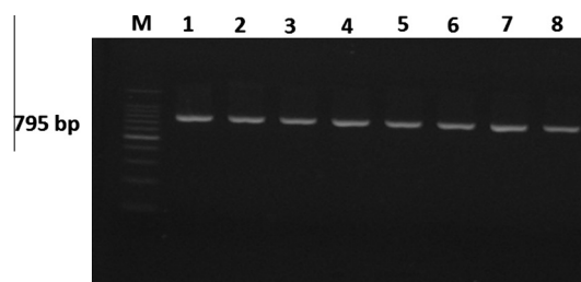
Fig. 1 Amplification of the tuf locus extracted from fish S. dysgalactiae isolates and S. dysgalactiae ATCC43078 yielded 795-bp when the primer pairs tuf1 and tuf2 were used. Lane M, marker; lane 1, S. dysgalactiae ATCC43078; lanes 2 and 3 Japanese fish isolates S. dysgalactiae ; lanes 4 and 5, Taiwanese fish isolates S. dysgalactiae ; lanes 6 and 7, Malaysian fish isolates S. dysgalactiae ; and lane 8, Indonesian fish isolate S. dysgalactiae .
