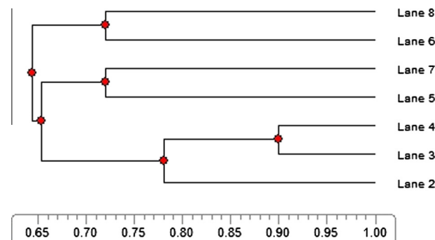
Fig. 3b Dendrogram constructed for BSFGE analysis using the UPGMA method with Phoretix 1D trial version.
