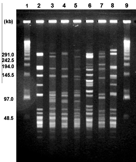
Fig. 3a The macrorestriction fragment profiles of DNAs digested with Sma I in seven representative isolates of S. dysgalactiae collected from fish. Lanes 1 and 9, marker DNA; Lane 2, KNH07807 (Japan); lane 3, 951003 (Taiwan); lane 4, 95985 (Taiwan); lane 5, PF880 (Malaysia); lane 6, T11358 (Indonesia); lane 7, PP1398 (Malaysia); lane 8, WSSN1609 (Malaysia).
