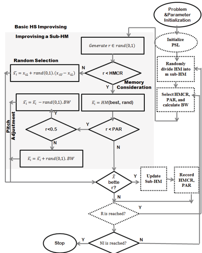
Fig. 1 DLHS Flowchart
