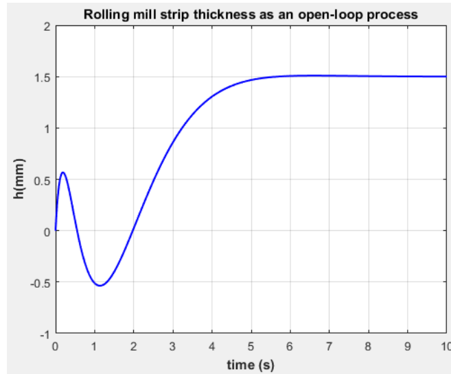
Figure 1: Step time response of the strip thickness.
