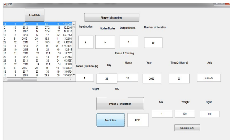
Figure 5: Proposed Application
