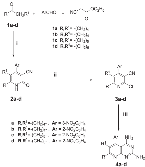
Scheme 1 Reagent and conditions: (i) \text{CH}_3\text{COONH}_4 , n-butanol, reflux 8 h; (ii) \text{POCl}_3 , dimethylaniline, reflux 10 h; (iii) guanidine HCL, \text{NaOC}_2\text{H}_5 , pyridine, reflux 5 h.
