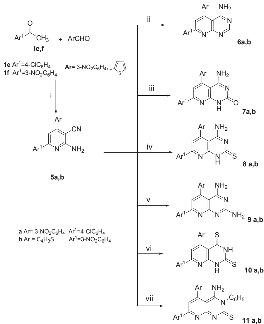
Scheme 2 Reagent and condition: (i) malononitrile, \text{CH}_3\text{COONH}_4 , n-butanol, reflux 8 h; (ii) formamide, oil bath, reflux 15 h; (iii) urea, oil bath, reflux 4 h; (iv) thiourea, oil bath, reflux 4 h; (v) guanidine HCL methanol, reflux 6 h; (vi) \text{CS}_2 , pyridine, reflux 15 h; (vii) PhCNS, DMF, TEA, reflux 10 h.
