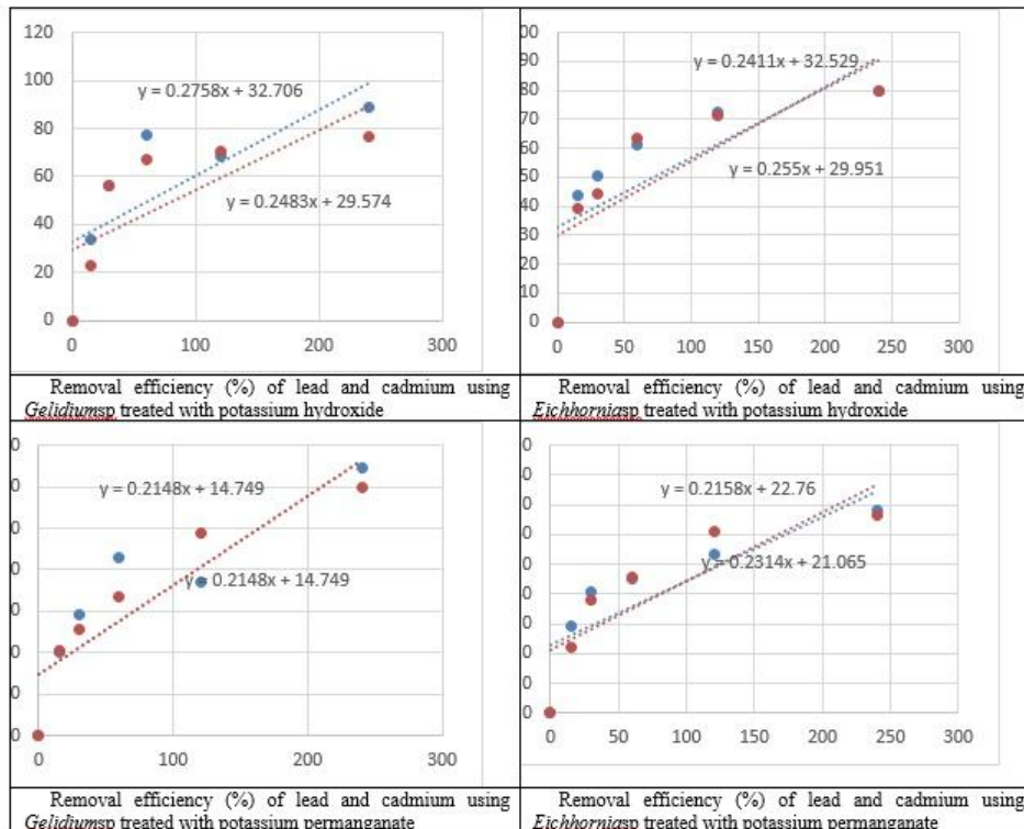
Fig. 3 — Removal efficiency (%) of lead and cadmium using Gelidium and Eichhornia sp treated by potassium hydroxide and potassium permanganate compounds against time (min.).
