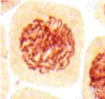
Normal Interphase
