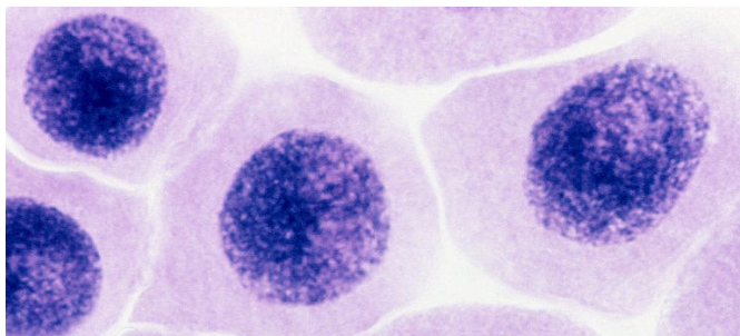
Interphase
