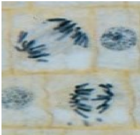
anaphase
