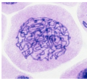
Prophase
