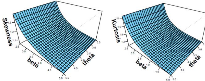
Figure 3. The skewness and kurtosis of the PTIR for \lambda = 0.5 and different values of \theta and \beta
