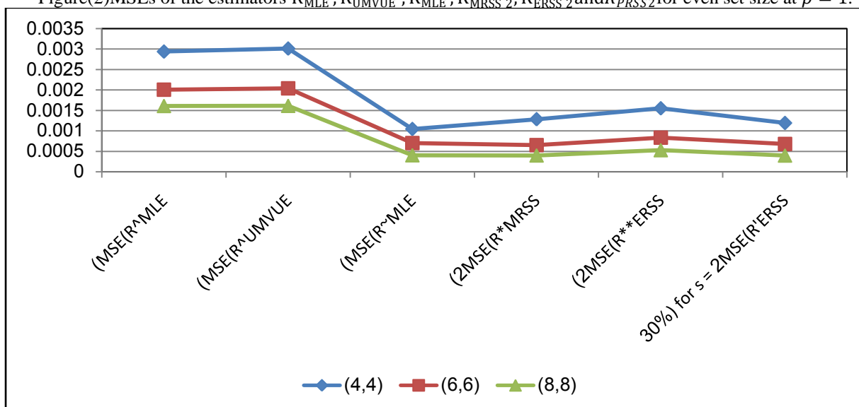
Figure(2)MSEs of the estimators \hat{R}_{MLE} , \hat{R}_{UMVUE} , \tilde{R}_{MLE} , R_{MRSS2}^* , R_{ERSS2}^{**} and \hat{R}_{PRSS2} for even set size at \rho = 1 .
