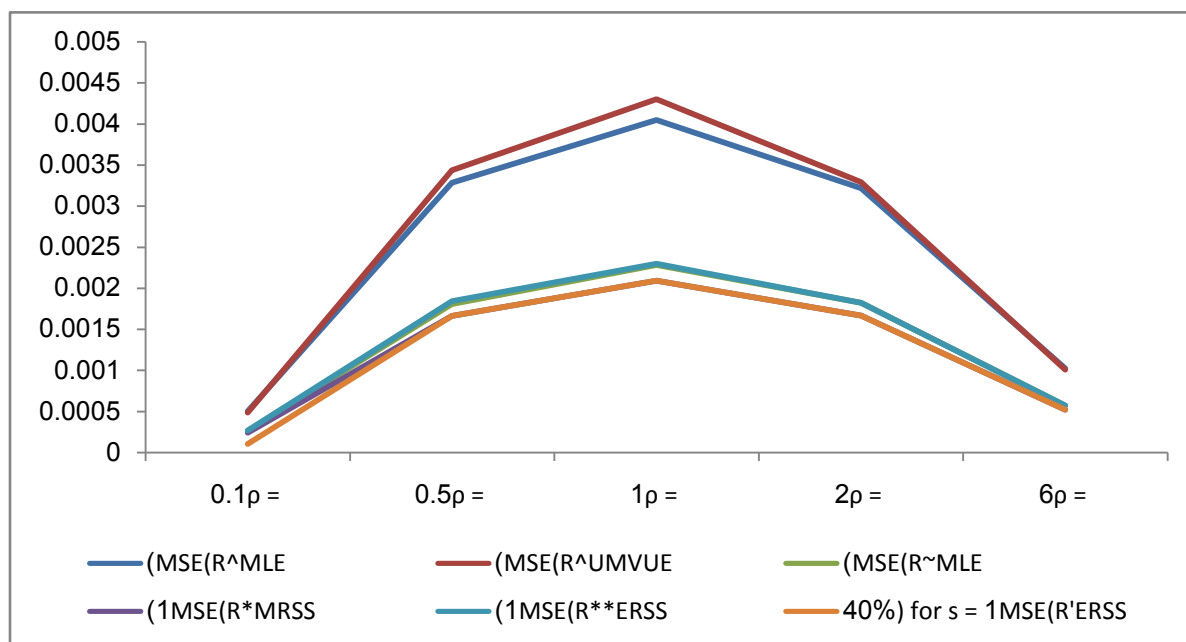
Figure(3)MSEs of the estimators \hat{R}_{MLE}, \hat{R}_{UMVUE}, \tilde{R}_{MLE}, R_{MRSS1}^*, R_{ERSS1}^{**} and \hat{R}_{PRSS1} at (n, m) = (3,3) .
