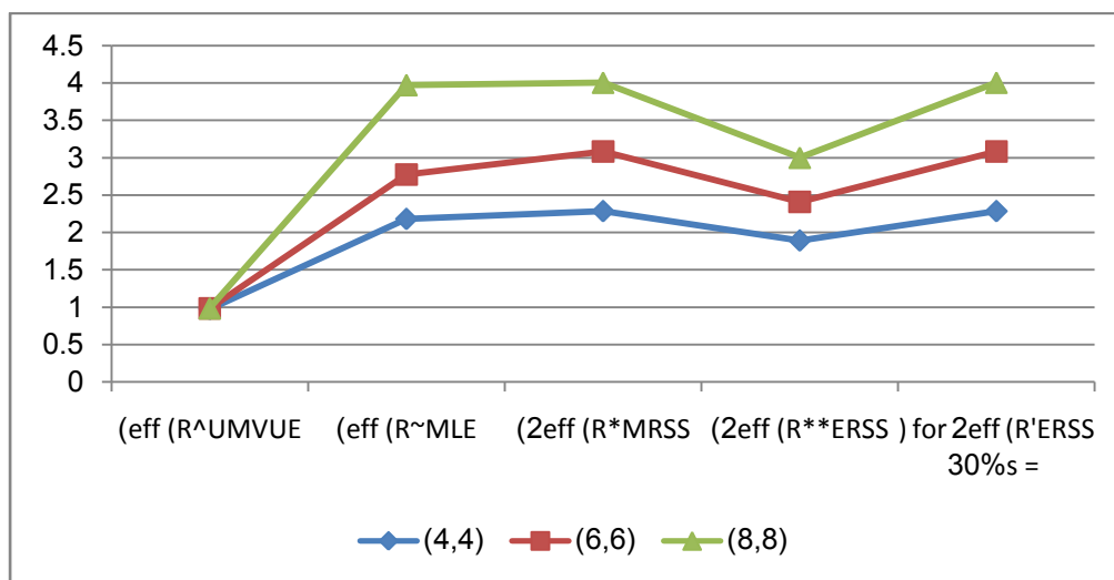
Figure(5)The efficiencies of the estimators \hat{R}_{UMVUE} , \tilde{R}_{MLE} , R_{MRSS2}^* , R_{ERSS2}^{**} and \hat{R}_{PRSS2} with respect to \hat{R}_{MLE} for even set size at \rho = 1 .
