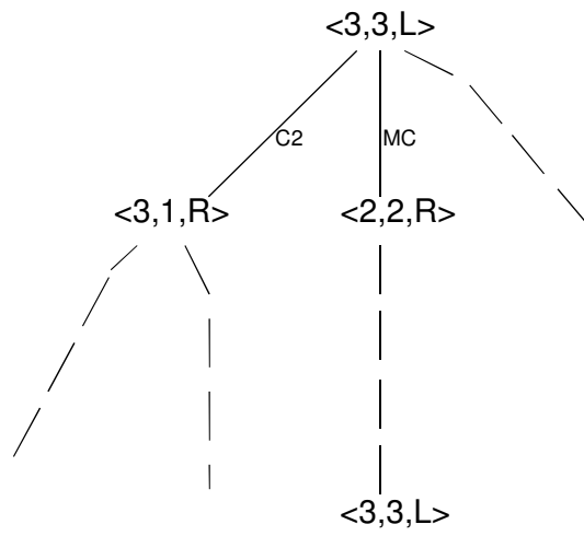
Search tree
