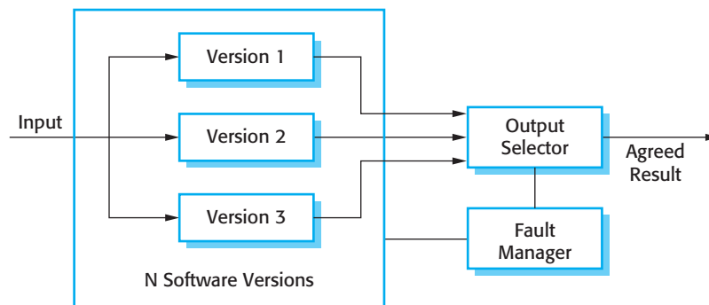
Figure 13.7 N-version programming
