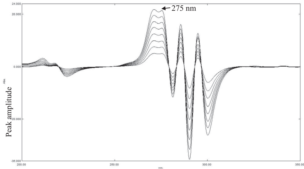
Fig. 5. First derivative of ratio spectra of DIM (10–45 \mu\text{g mL}^{-1} ) using normalized CIN spectrum as a divisor.
