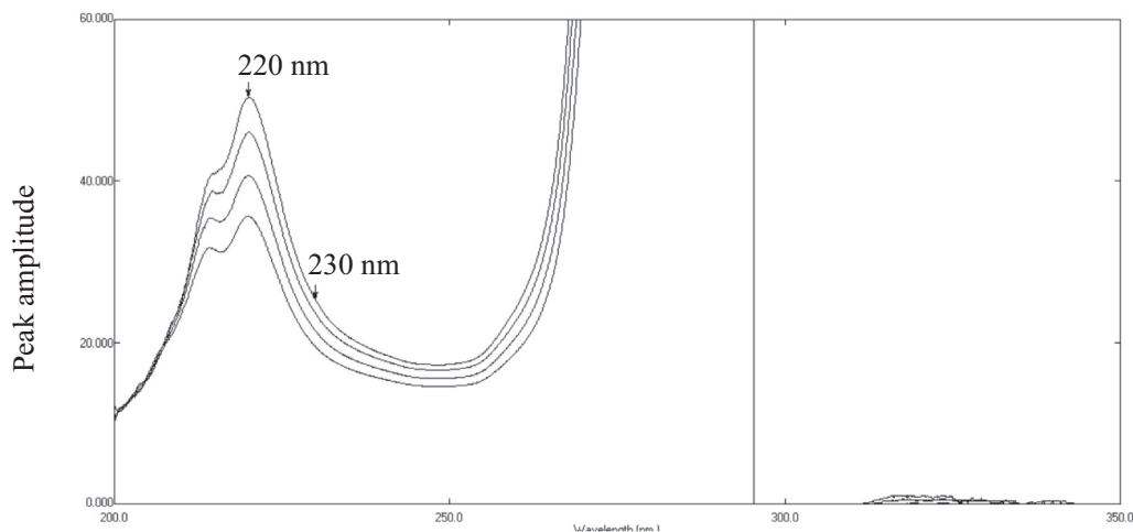
Fig. 6. Ratio spectra of synthetic mixture of DIM 15.0 \mu\text{g mL}^{-1} and CIN 10.0 \mu\text{g mL}^{-1} , after addition of different DIM concentrations (10.0–25.0 \mu\text{g mL}^{-1} ), using normalized CIN spectrum as a divisor.
