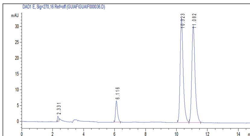
Fig. 5 Chromatogram of pharmaceutical sample solution containing 30 \mu\text{g mL}^{-1} of AMB and 100 \mu\text{g mL}^{-1} of each of GUA enantiomers, separated on Lux cellulose-2 column, using ethanol/hexane (15 : 85 v/v) as mobile phase at 1.2 mL min -1 flow rate and column temperature at 19 °C.
