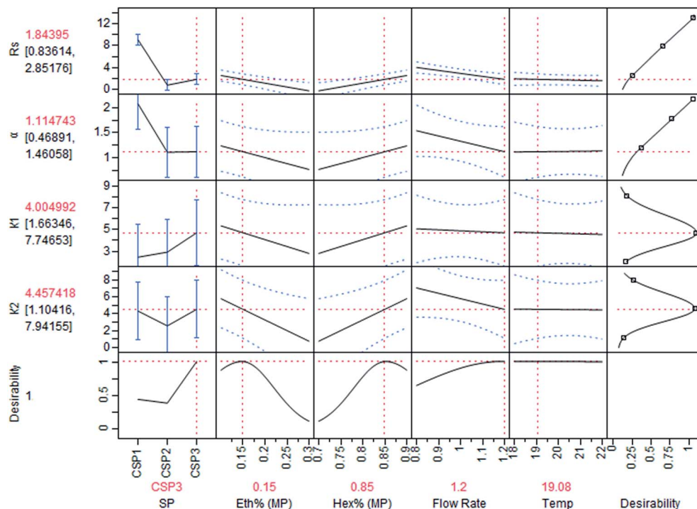
Fig. 4 Prediction profiler showing the effect of each factor on the studied responses; resolution ( R_s ), selectivity factor ( \alpha ), capacity factors ( K'_1 and K'_2 ) for GUA enantiomers 1 and 2, respectively.
