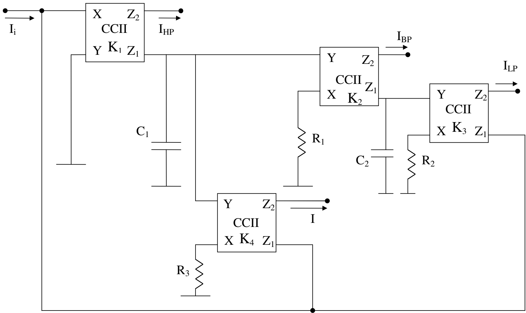
Fig. 2 Universal correct mode filter (Corrected)
