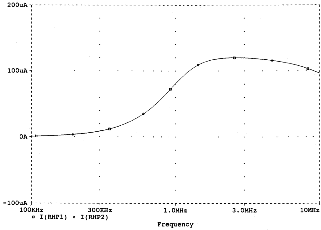
Fig. 11. The highpass output current.
