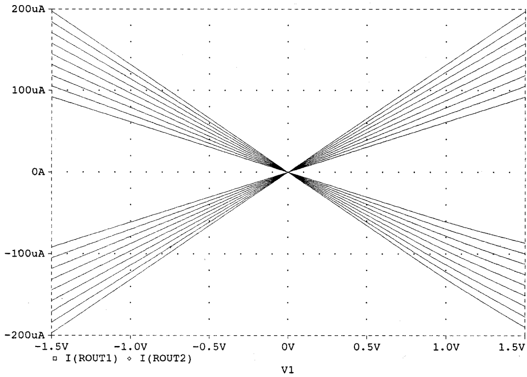
Fig. 3(b). The I-V characteristics of the output currents of the BOTA with Vc as a parameter.
