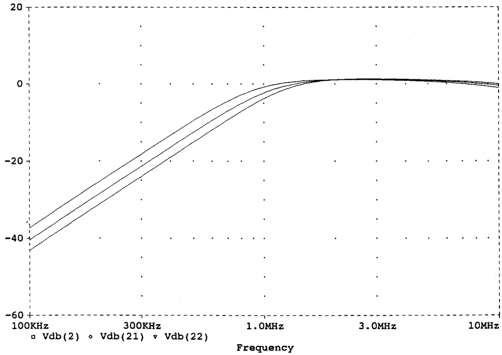
Fig. 9. The magnitude response of the voltage mode highpass output.
