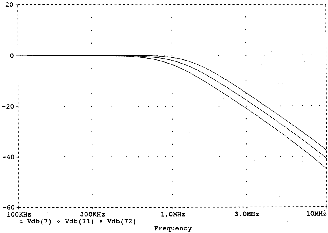
Fig. 8. The magnitude response of the voltage mode lowpass output.
