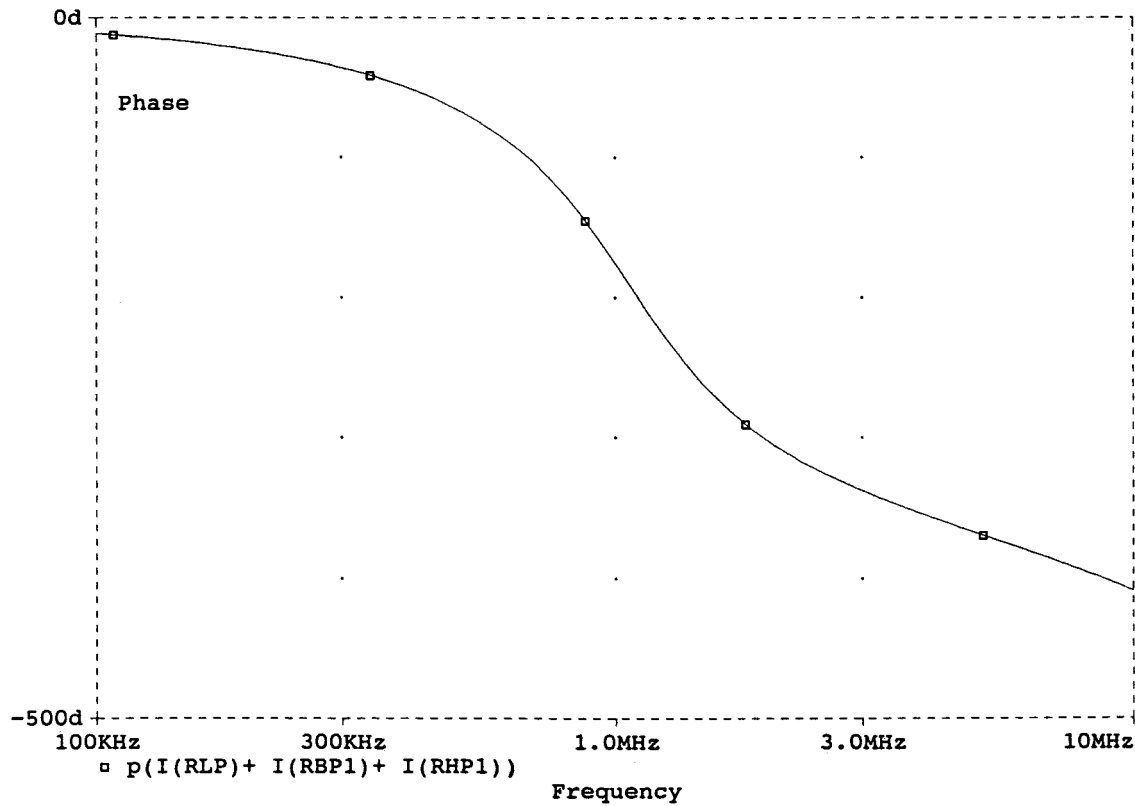
Fig. 13. The phase response of the allpass output current.
