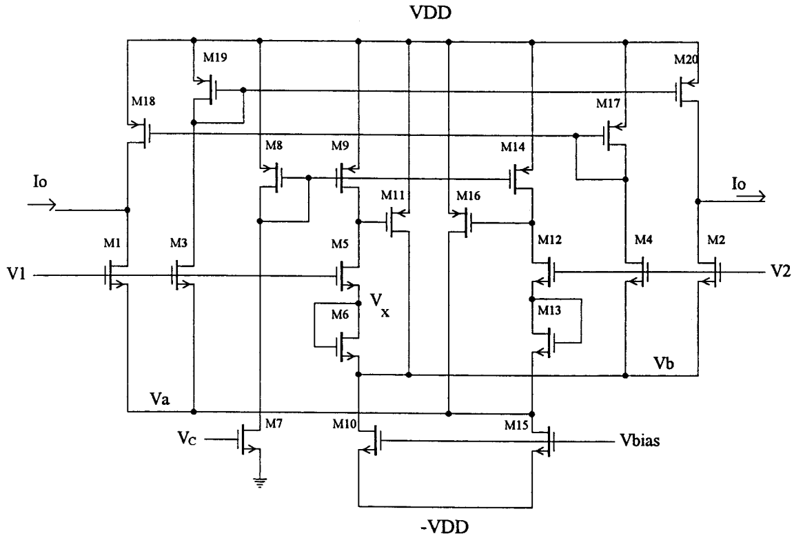
Fig. 2. The CMOS circuit of the BOTA.
