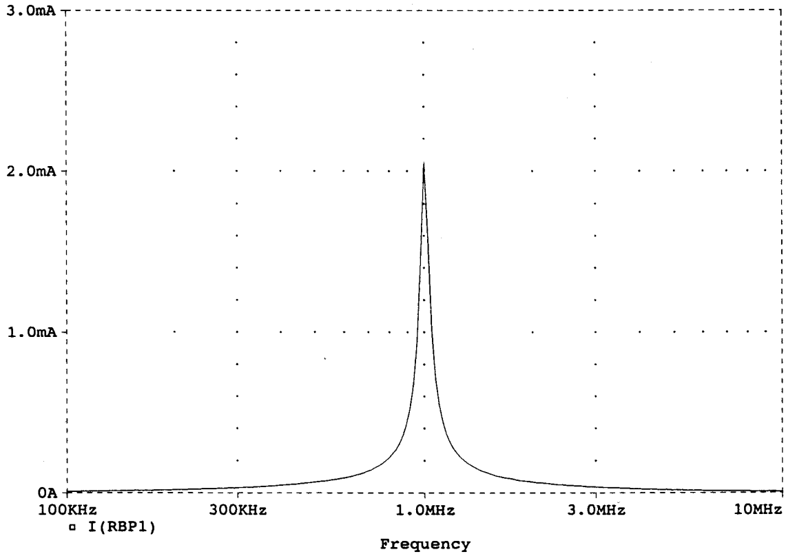
Fig. 7. The bandpass output current.
