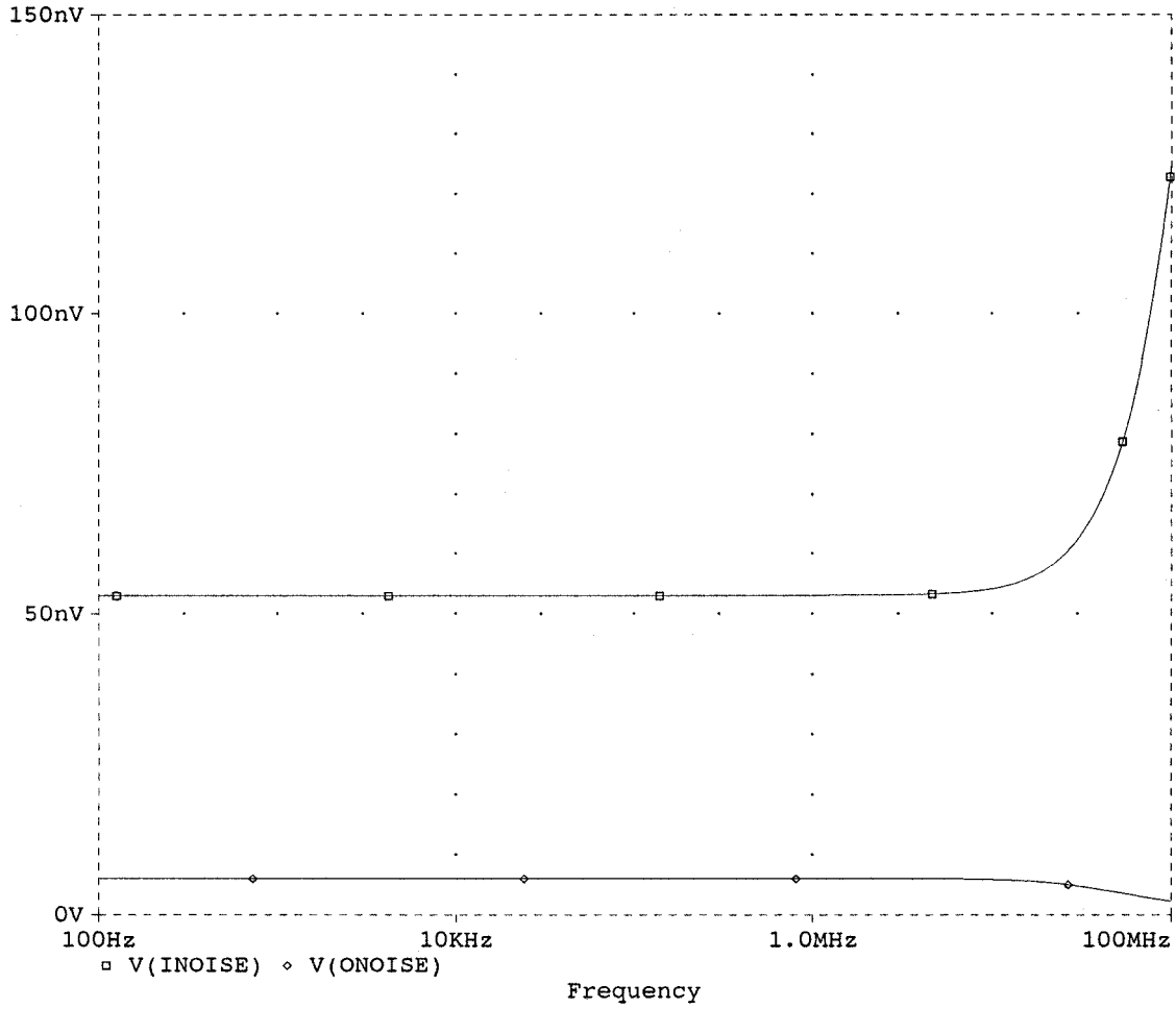
Fig. 4(c). The output-referred and input referred noise voltage spectral densities for the BOTA when terminated by 1 K \Omega .
