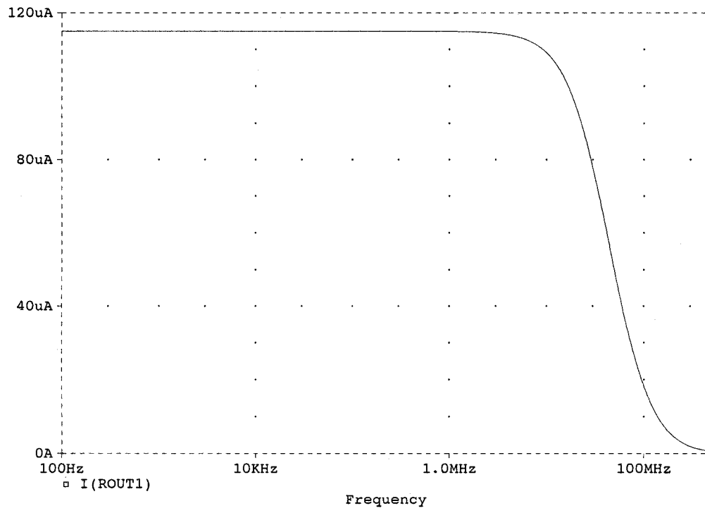
Fig. 4(a). The magnitude response of the proposed BOTA.
