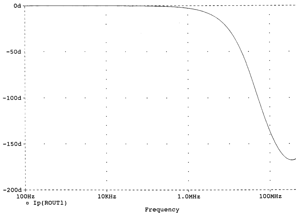
Fig. 4(b). The phase response of the proposed BOTA.
