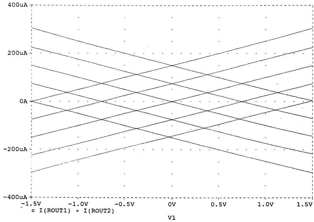
Fig. 3(a). The I-V characteristics of the output currents of the BOTA.
