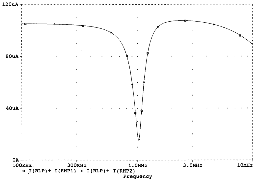
Fig. 12. The magnitude response of the notch output current.
