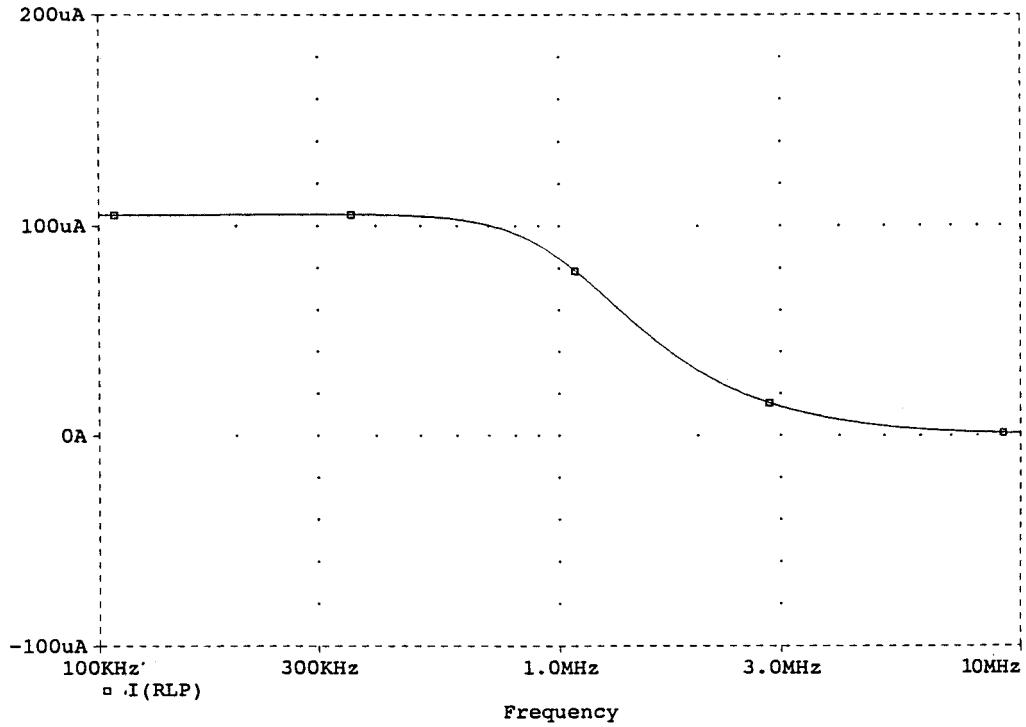
Fig. 10. The lowpass output current.
