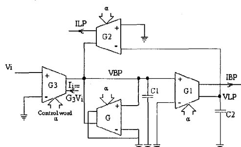
Fig. 8: DCBOTA-C Active Filter
