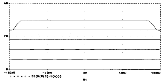
Fig. 7: dB Gain of The Proposed VGA at Gain Step = 6 dB
