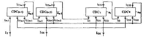
Fig. 2: Proposed CDN Block Diagram
