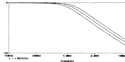
Fig. 10: The Magnitude Response of the Voltage-Mode Lowpass Output
