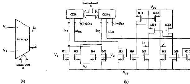
Fig. 1: Proposed DCBOTA (a) Symbol (b) CMOS Realization
