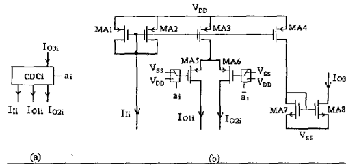
Fig. 3: Proposed CDC (a) Symbol (b) CMOS Realization
