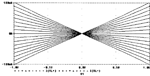
Fig. 4: DC Transfer Characteristics of The Proposed DCBOTA
