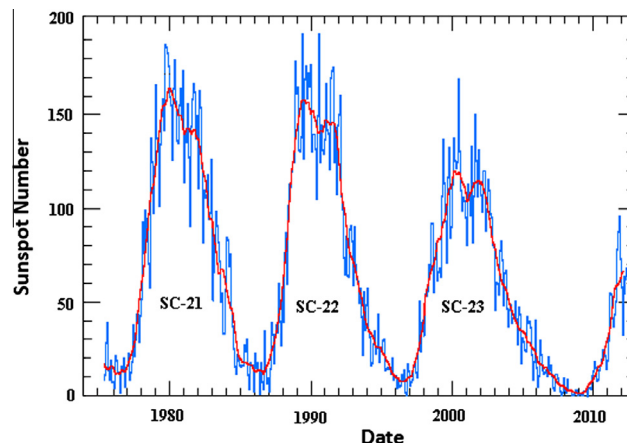
Fig. 1 The monthly means (blue) and monthly smoothed (red) sunspot numbers for the latest three cycles and ascending phase, the data given from, http://sidc.oma.be/sunspot-data .
