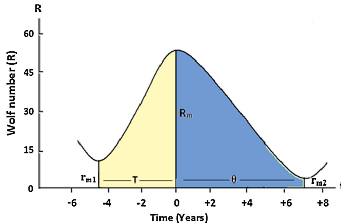
Fig. 2 Schematic diagram of sunspot curve of the 11-year cycle according to Waldmeier Laws [14].
