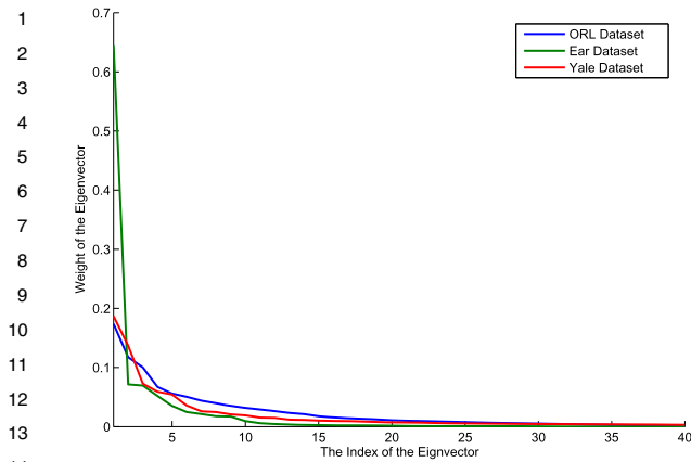
Fig. 11. The robustness of the first 40 eigenvectors of the LDA technique using ORL 32×32 , Ear 32×32 , and Yale 32×32 datasets.
