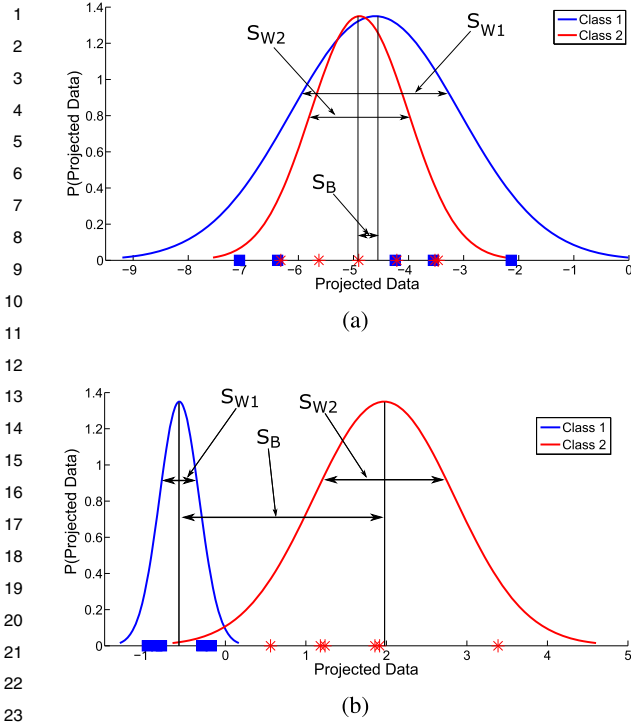
Fig. 4. Probability density function of the projected data of the first example, (a) the projected data on V_1 , (b) the projected data on V_2 .
