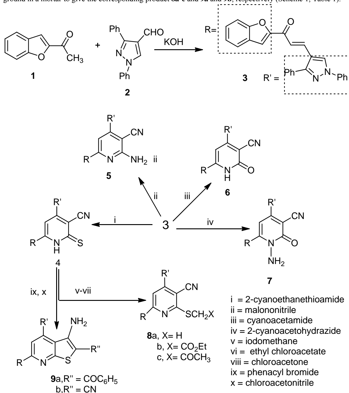
Scheme 1
