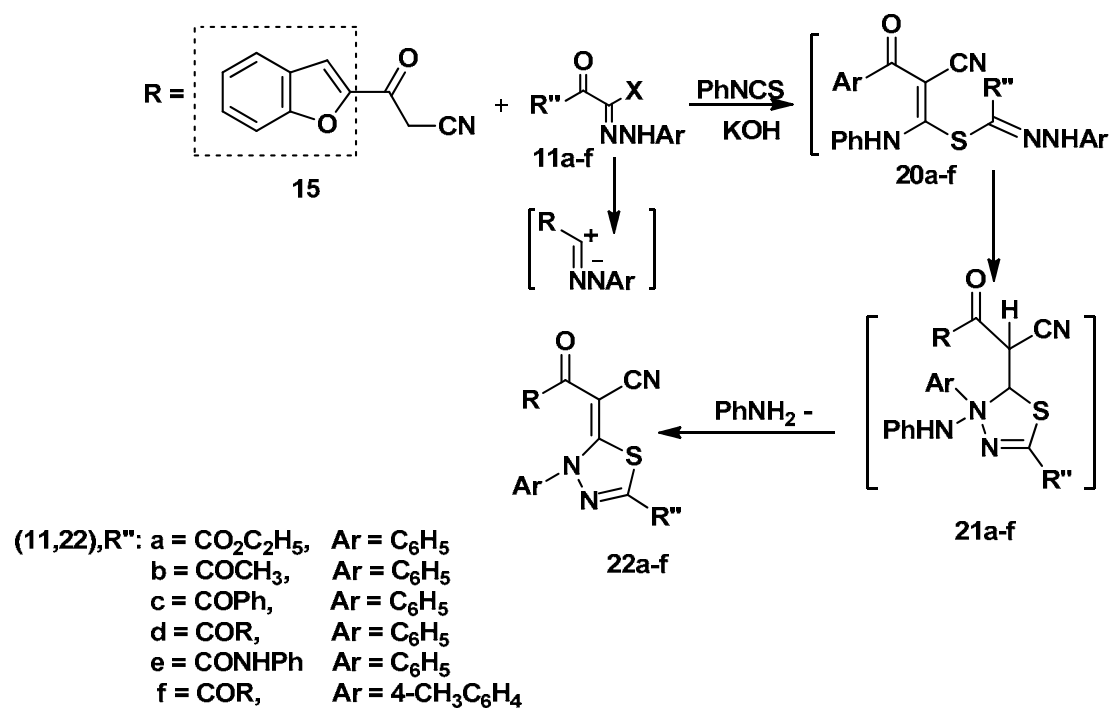
Scheme 4
