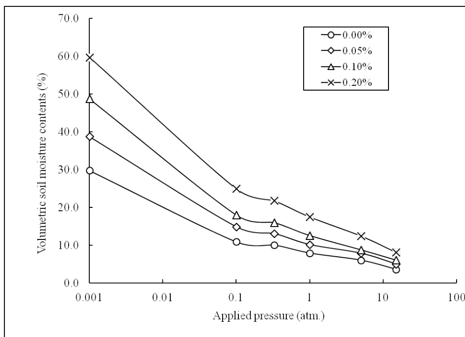
Fig. 1: Soil moisture characteristic curves of sandy- amended soil treated with different hydrogel levels.
