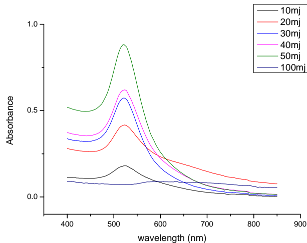
Figure 6. The absorbance spectrum of gold nanoparticles prepared in pure water at (10 - 100 mJ).
