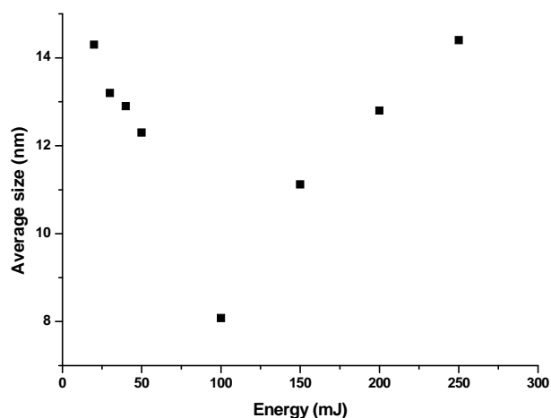
Figure 5. The relation between the energy and the average size.
