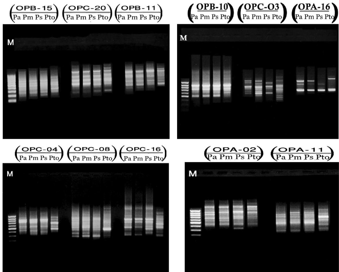
Fig. 4. RAPD fingerprinting patterns of four species of Panocratium generated by 11 primers. PA – Panocratium arabicum ; PM – P. maritimum ; PS – P. sickenbergeri ; PT – P. tortuosum ; M – 100 kb ladder.
