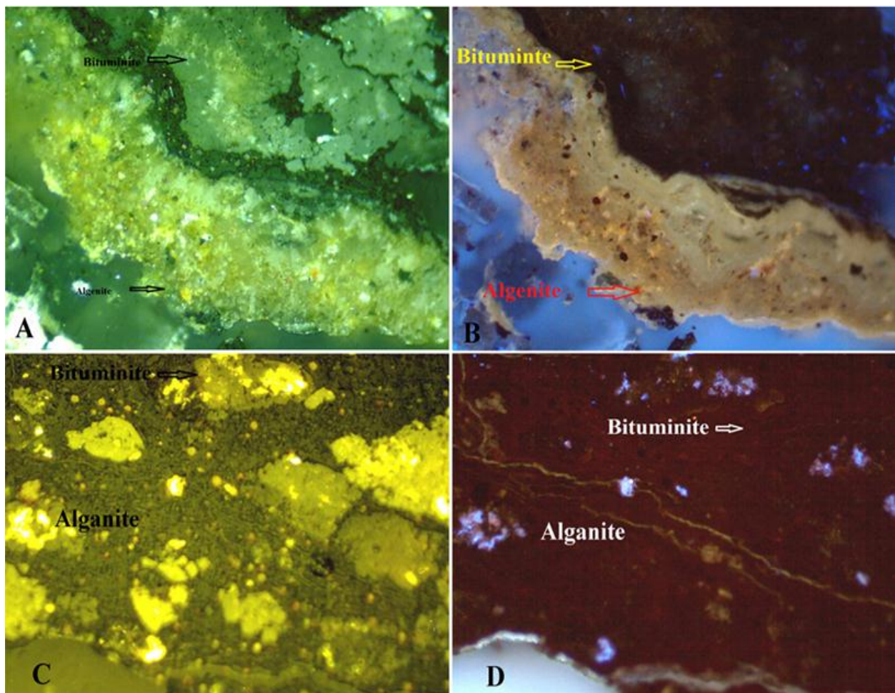
Fig-8. P Petrographic characteristics of Sargelu oil shale samples from Banik area, Northern Iraq. Alginites and bituminite A & C (Blue light) X200 B & D (Reflected light) X200
