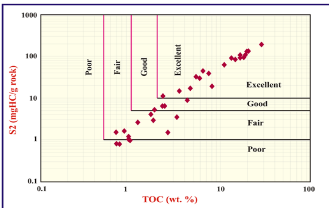
Fig-3. TOC wt% versus S2 plot of Sargelu and Naokelekan formations indicates their hydrocarbon potentialities.
