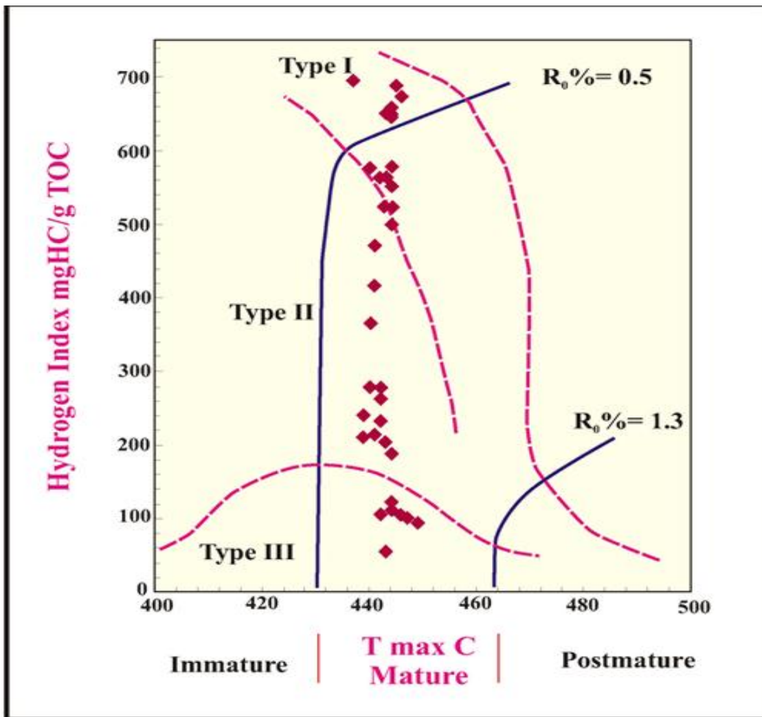
Fig-5. Kerogen plots for HI vs. T_{max} of the samples of Sargelu and Naokelekan formations of the Banik section.
