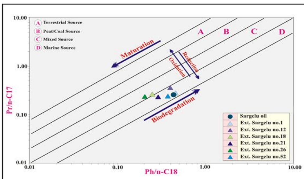
Fig-7. Pr/n-C17 versus Ph/n-C18 of the Sargelu Formation extracts and the oil samples.
