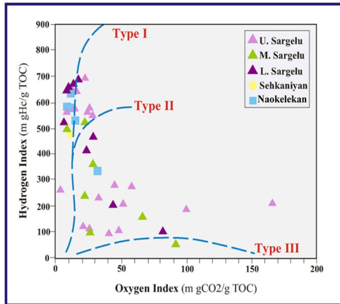
Fig-2. Van Krevelen diagram, showing Rock-Eval Hydrogen Index vs. Oxygen Index for the analyzed samples of the study area (adapted from Espitalié, et al. [21])
