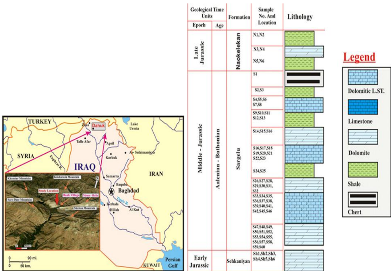
Fig-1. Location map and the stratigraphic column of Jurassic rocks crop-out in the Banik area, North Iraq indicating the collected samples.
