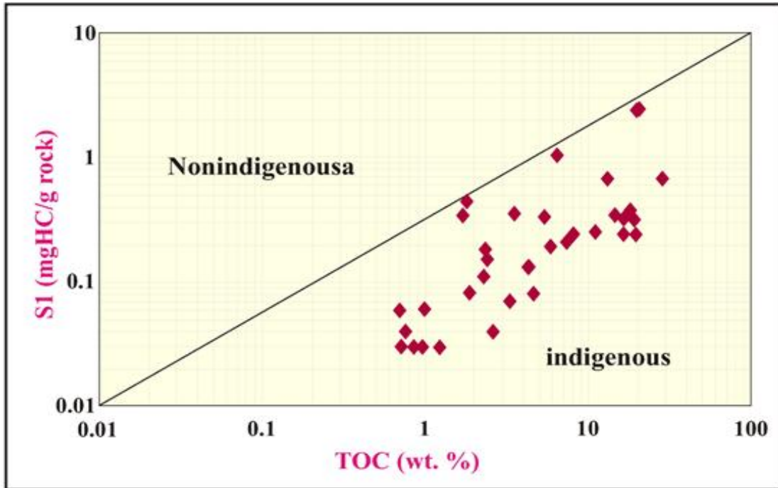
Fig-4. S1 versus TOC for Sargelu and Naokelekan formations in Banik section (modified after Hunt [22])
