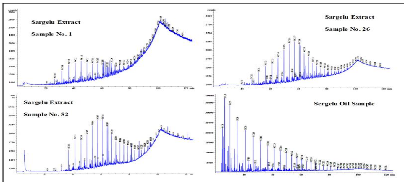
Fig-6. Gas Chromatograms of the rock extract of the Sargelu Formation and its oil sample from North Iraq.
