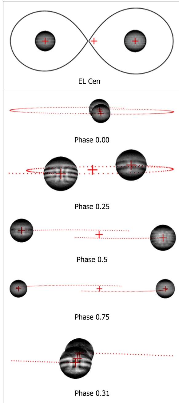
Figure 8. Top panel: Roche Lobe configuration. Bottom: The description of the model solution at different orbital phases for Cen.
