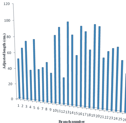
Fig. 2: Histogramme representing length of primary branches of S. sophera at the age of 24 weeks
