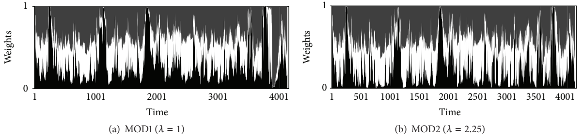
FIGURE 8: Dynamics of the adaptive belief system: chartists (black region), fundamentalists (grey region), and inactive traders (white region) for (a) the MOD1 and (b) the MOD2, respectively.
