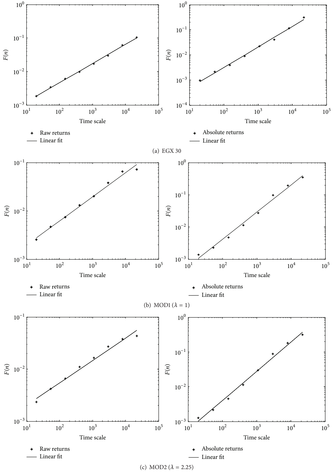
FIGURE 7: Estimation of self-similarity parameter H for raw and absolute returns, respectively, for (a) the EGX 30, (b) the MOD1, and (c) the MOD2, respectively. To estimate the self-similarity parameter we follow Peng et al. [57] and perform a detrended fluctuation analysis (DFA). A linear relationship on a log-log scale plot indicates the presence of power-law scaling. The slope of the line relating \log(F(n)) to \log(n) is the estimated scaling exponent, n = \{2^3, \dots, 2^{10}\} . The scaling exponent H_r yields a value of 0.57 \pm 0.025 for the EGX 30, 0.49 \pm 0.067 for the MOD1, and 0.43 \pm 0.054 for the MOD2, which are close to the theoretically expected value of the white-noise process. The scaling exponent H_{|r|} reveals a value of 0.81 \pm 0.056 for the EGX 30, 0.88 \pm 0.087 for the MOD1, and 0.84 \pm 0.071 for the MOD2, which indicate persistent long-range (power-law) autocorrelations in absolute returns for the three time series under investigation.
