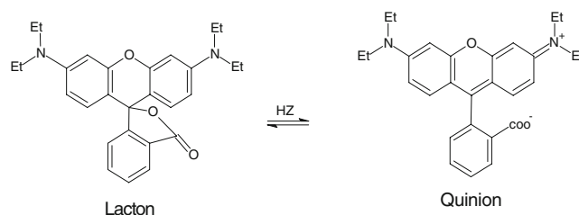
Fig. 10 Equilibrium between lactone and quinone form in the polar solvent
