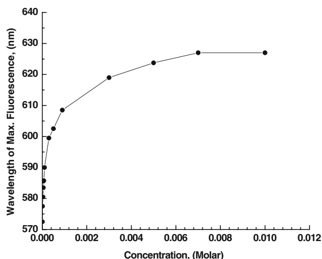
Fig. 5 The effect of concentration on the wavelength of the maximum fluorescence emission of Rhodamine B in ethanol
