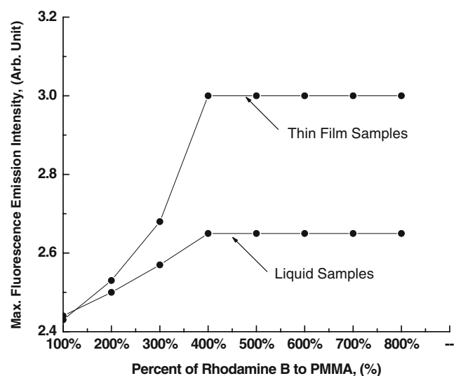
Fig. 7 The maximum fluorescence intensity of Rhodamine B ( C=3 \times 10^{-4} M) to PMMA ( C=8 \times 10^{-4} M) for thin film and liquid samples at different ratios
