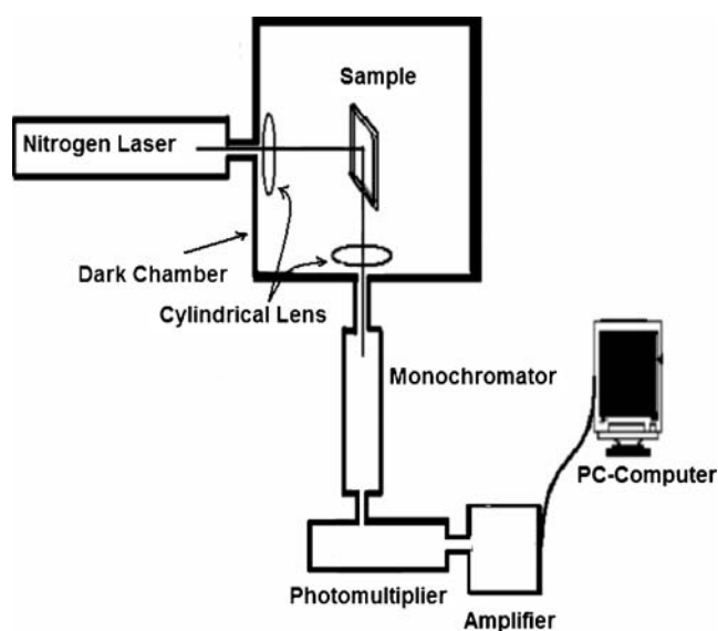
Fig. 1 Laser Induced Luminescence (LIF) set-up
