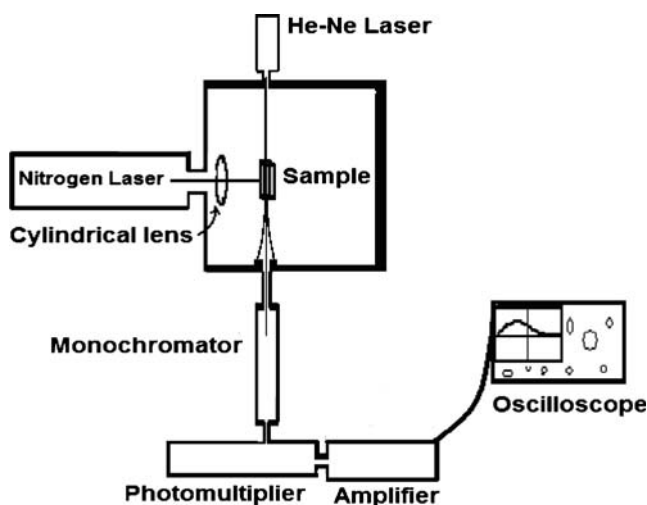
Fig. 2 Dual beam thermal lens technique
