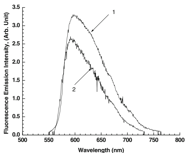
Fig. 6 The effect of solvent on the maximum fluorescence emission intensity of Rhodamine B with concentration 3 \times 10^{-4} M. Curve (1) in ethanol and curve (2) in THF
