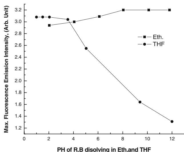
Fig. 8 The effect of pH on the fluorescence emission intensity of Rh B C=3 \times 10^{-4} M dissolving in ethanol and in THF
