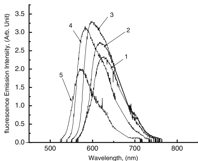
Fig. 3 The fluorescence emission intensity of Rhodamine B in ethanol as a function of wavelengths at different concentrations in curves, (1) C=7 \times 10^{-3} M, (2) C=3 \times 10^{-3} M, (3) C=3 \times 10^{-4} M, (4) C=5 \times 10^{-5} and (5) C=1 \times 10^{-5} M
