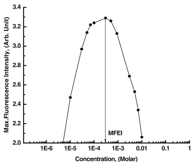
Fig. 4 The effect of concentration on the maximum fluorescence emission intensity of Rhodamine B in ethanol
