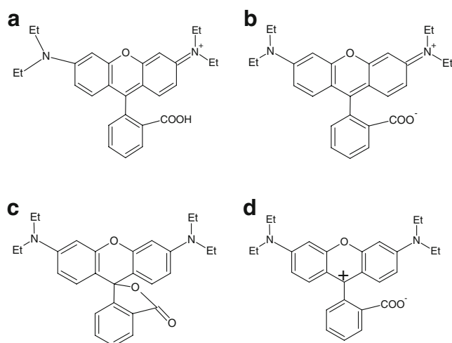
Fig. 9 Different formula of Rhodamine: a cationic, b quinonic, c Lactonic and d zwitterionic
