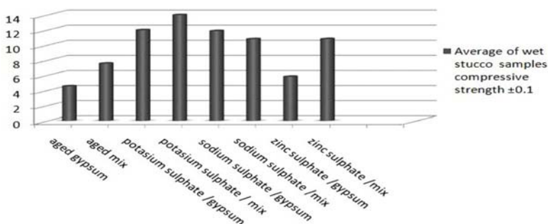
Fig. 15. All stucco samples achieved average of compressive strength of wet stucco samples more than the aged stucco samples, especially \text{K}_2\text{SO}_4 and \text{Na}_2\text{SO}_4 , which may be a result of retransformation of anhydrite to gypsum. The increasing ratio in \text{ZnSO}_4 \cdot 7\text{H}_2\text{O} gypsum stucco samples was very low, and may relate to the non-interlocked gypsum crystals.
