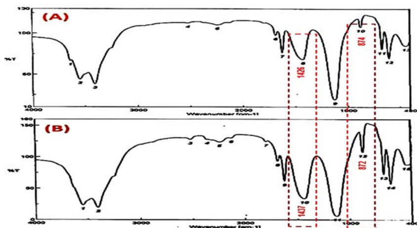
Fig. 2. FTIR spectra from the gypsum lime stucco samples (A) after 1 month (B) after 10 months, bands related to \text{CO}_3 prove the results of XRD analysis.
