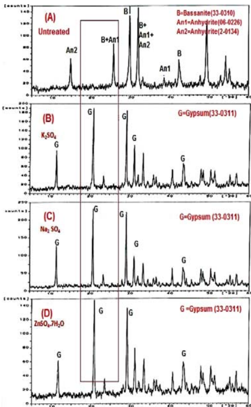
Fig. 5. The X-ray diffraction patterns of the treated gypsum stucco samples with the selected sulphate activators solutions, after more than 28 days, in comparison with the untreated sample, the patterns indicate the appearance of gypsum and the approximate disappearance of anhydrite
