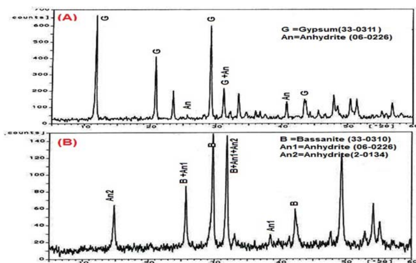
Fig. 3. The X-ray diffraction pattern of the gypsum stucco samples that were exposed to a temperature of 300^\circ\text{C} \pm 10 for six hours, in comparison with the non-heated gypsum sample. The figure shows the transformation of gypsum content to anhydrite and other intermediate phases of gypsum.
