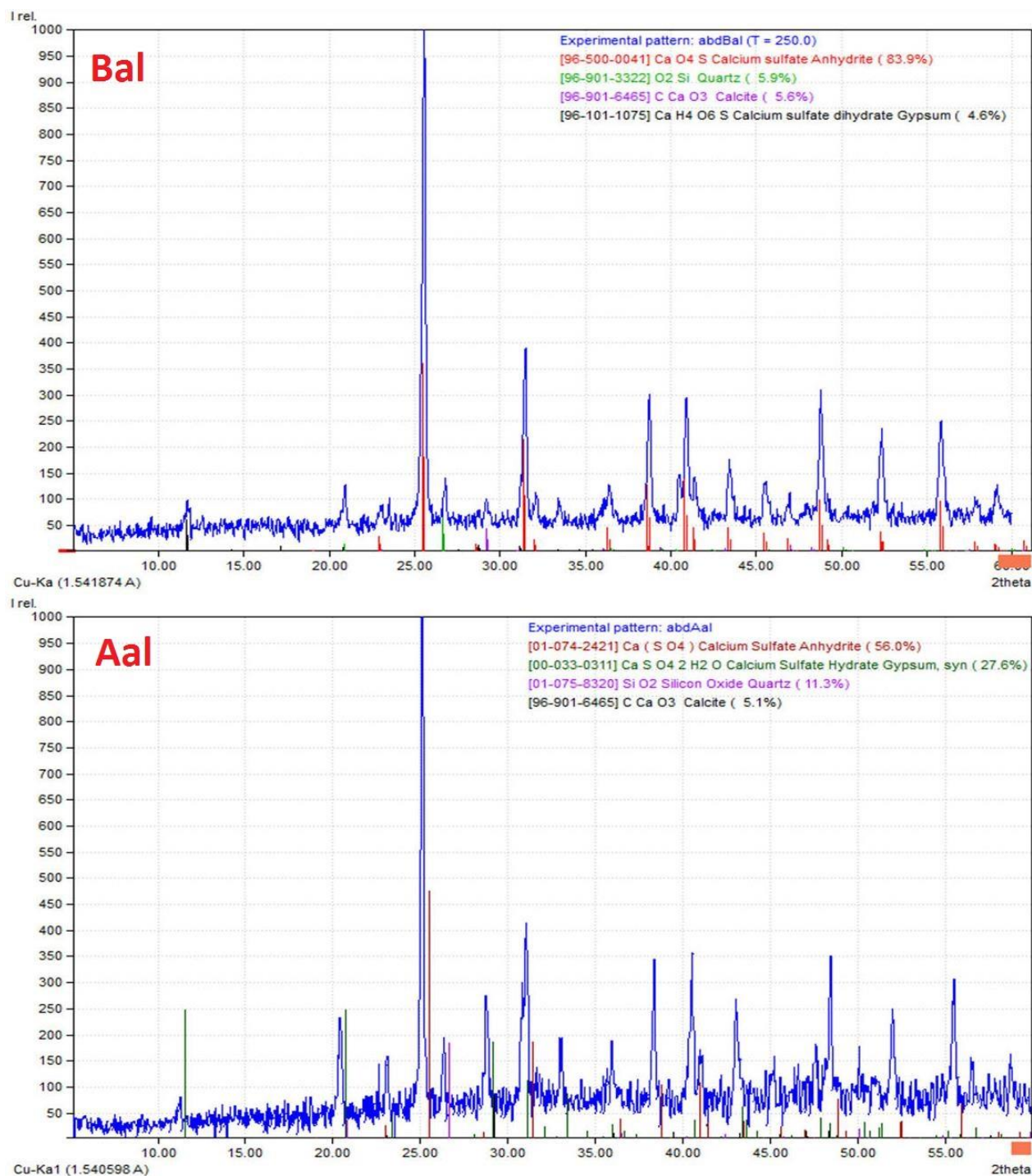
Figure 3 X-ray diffraction patterns of the archaeological stucco sample taken from the Al Alayaa minaret. (Bal) before the application of K_2SO_4 solution, (Aal) after the application of K_2SO_4 solution. The results show the effect of potassium sulphate solution for increasing of anhydrite conversion to gypsum.
