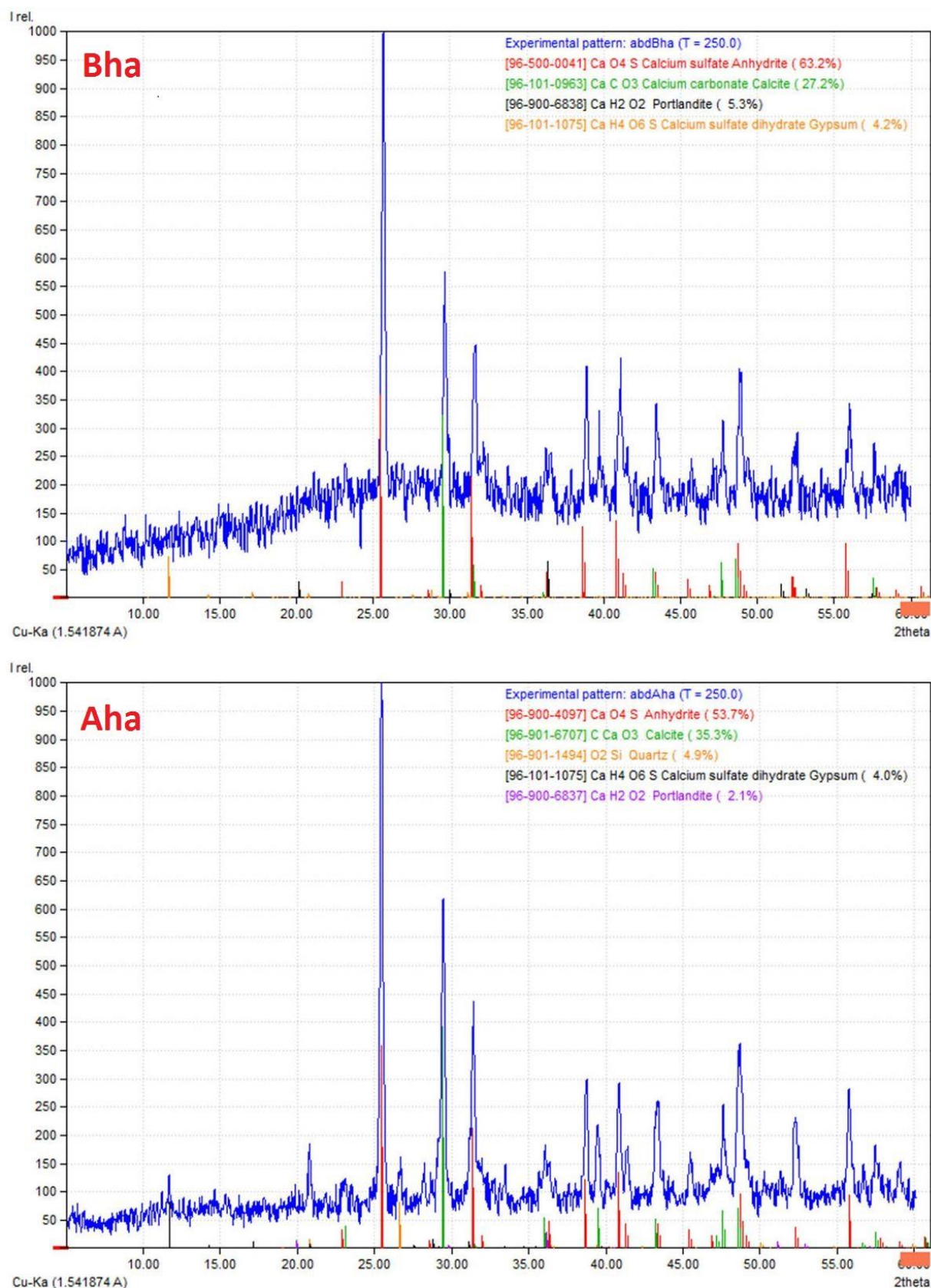
Figure 2 X-ray diffraction patterns of the archaeological stucco sample taken from the Habu temple plaster. (Bha) before the application of K_2SO_4 solution, (Aha) after the application of K_2SO_4 solution. There is not any remarkable detected conversion from anhydrite to gypsum.
