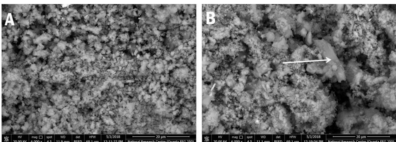
Figure 7 Scanning electron micrographs of the untreated sample (A) and the treated sample (B) of the Al Alaaya stucco with K_2SO_4 solution showed the appearance of the interlocked needle-like crystals, this may be related to the reformation of gypsum crystals.
