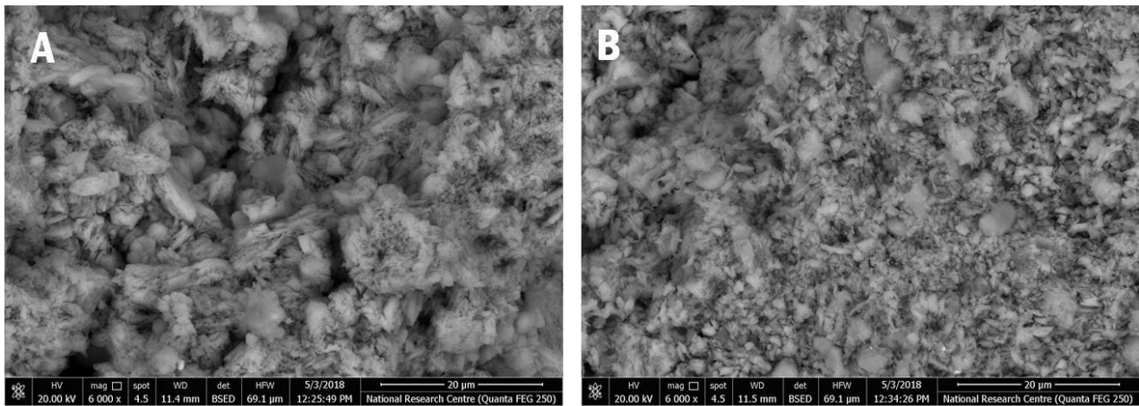
Figure 5 Scanning electron micrographs of the untreated sample (A) and the treated sample (B) of the Habu plaster with K_2SO_4 solution show that no noticeable change in the crystallographic forms.
