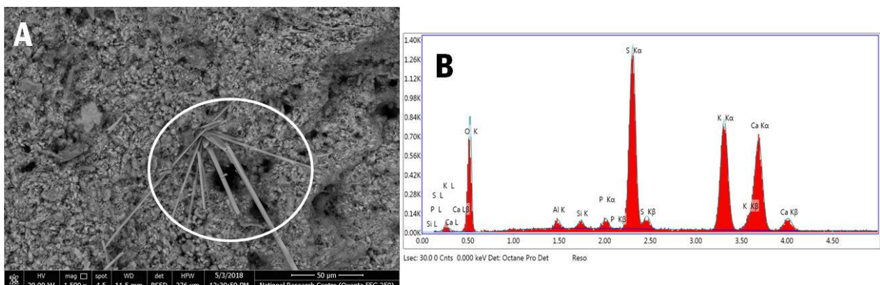
Figure 6 (A) Scanning electron micrograph of the efflorescence spots of the elongated crystals which were detected on the Habu sample surface. (B) EDX spectra results of the elongated crystals show the appearance of (K), (S) and (O) elements which may confirm that it is potassium sulphate salt.
