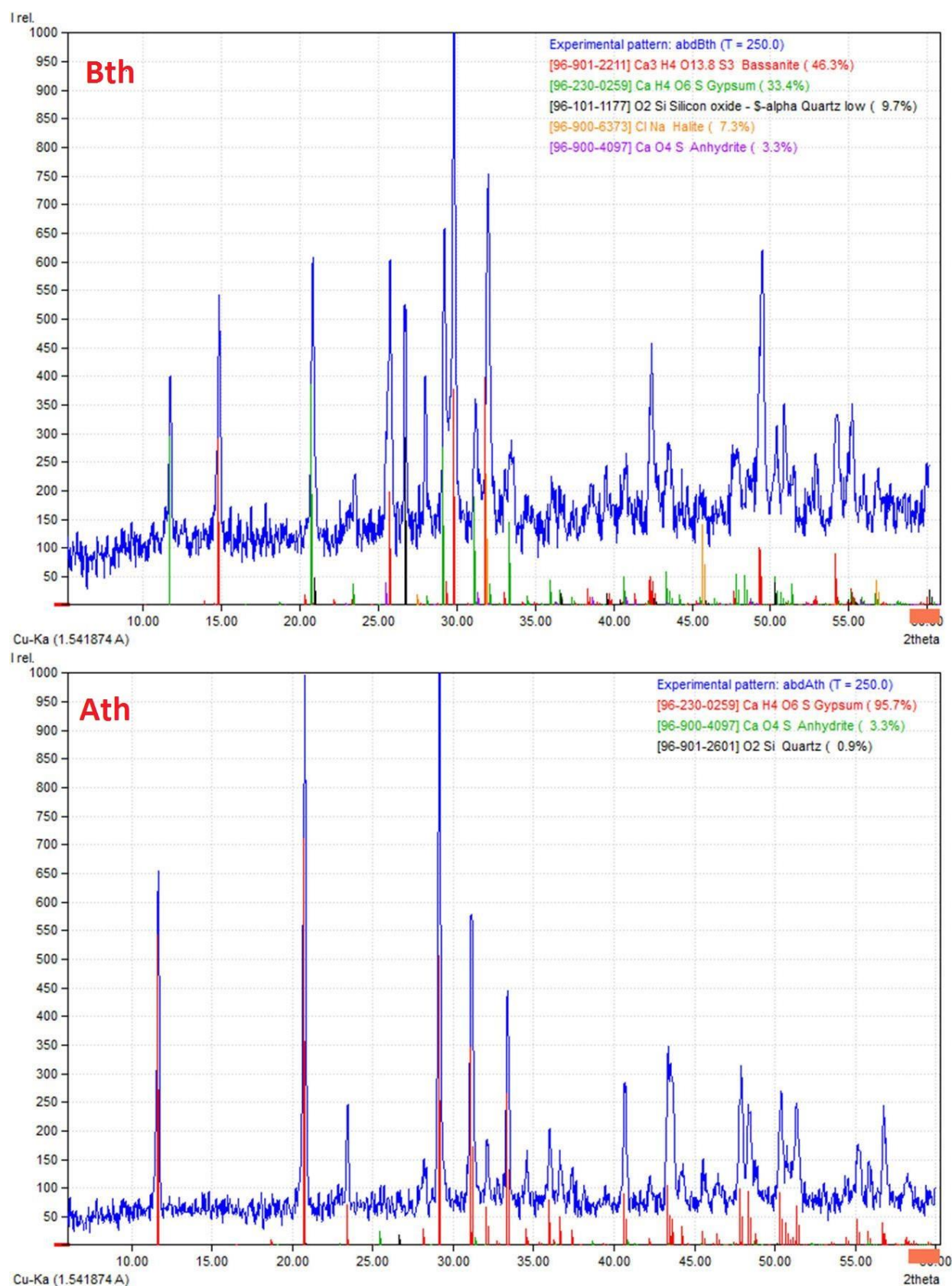
Figure 4 X-ray diffraction patterns of the archaeological stucco sample taken from the Egyptian national theater. (Bth) before the application of K_2SO_4 solution, (Ath) after the application of K_2SO_4 solution. The results show the disappearance of bassanite as well as the remarkable increase of gypsum.
