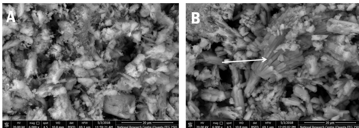
Figure 8 Scanning electron micrographs of the untreated sample (A) and the treated sample (B) of the Egyptian national theater with K_2SO_4 solution show the obvious appearance of the interlocked needle-like crystals which confirms the conversion of the intermediate phase to gypsum crystals.
