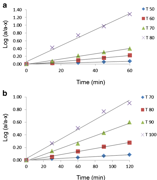
Fig. 5 Effect of different heating times with 0.1 M HCL and 0.1 M NaOH on the rate of degradation of a AZL (25 µg mL -1 ) and b CLT (20 µg mL -1 ), respectively
