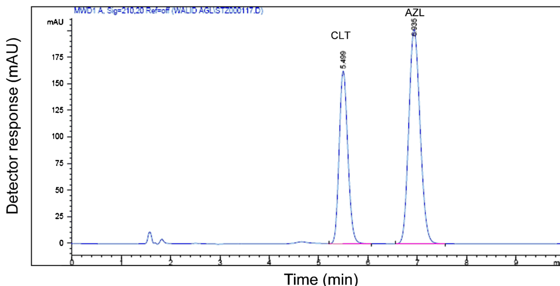
Fig. 2 Typical LC chromatogram for Edarbacyclor ® tablets—24 \mu\text{g mL}^{-1} AZL (6.9 min) and 15 \mu\text{g mL}^{-1} of CLT (5.5 min) under the described chromatographic conditions
