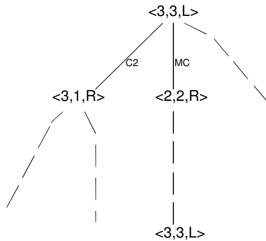
Search tree
