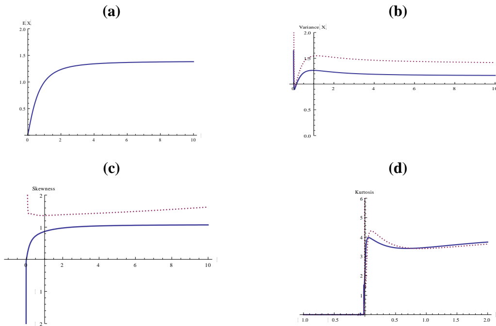
Figure 2: Illustrates the shapes of (a) the expectation value E(X) of S'GLD(\alpha, \beta, \lambda) , when \lambda \in (0, 10) , \beta = 1 and \alpha = 2 (Thick line) and \alpha = 1 (dashed line). (b) the variance \text{var}(X) , when \lambda \in (0, 10) , \beta = 2 and \alpha = 1 (Thick line) and \alpha = 1.5 (dashed line). (c) the skewness coefficient, when \lambda \in (-1, 10) , \beta = 1 and \alpha = 1 (Thick line) and \alpha = 2 (dashed line). (d) the kurtosis coefficient, when \lambda \in (-1, 10) , \beta = 1 and \alpha = 1 (Thick line) and \alpha = 1.5 (dashed line).
